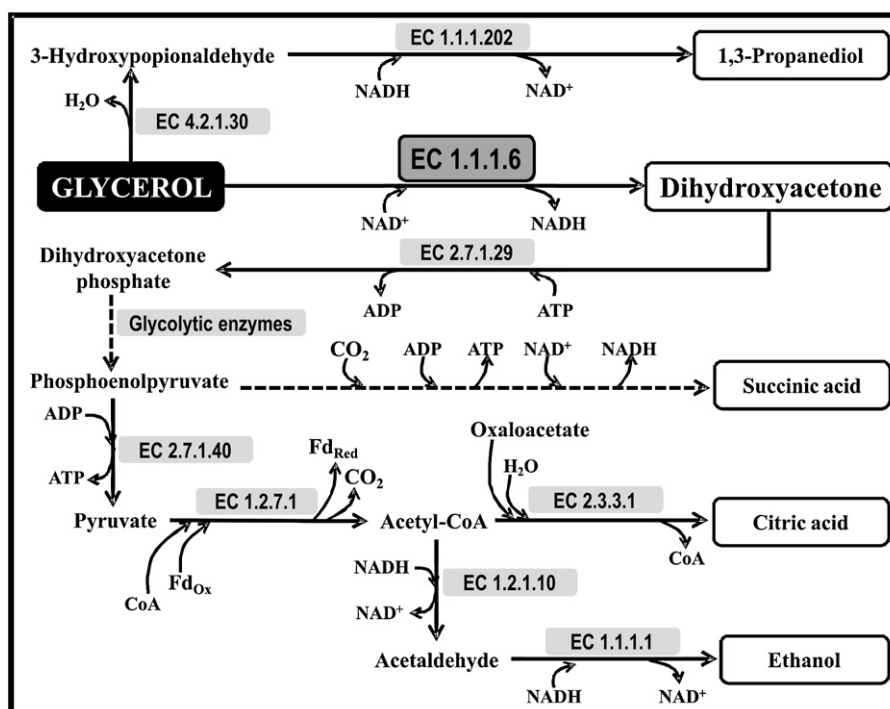
Fig. 1. Schematic diagram of the enzymes (EC number) and pathways involved in the biochemical transformation of Gro. EC 1.1.1.1, alcohol dehydrogenase; EC 1.1.1.6, GroDHase; EC 1.1.1.202, 1,3-propanediol oxidoreductase; EC 1.2.1.10, acetaldehyde dehydrogenase; EC 1.2.7.1, pyruvate synthase; EC 2.3.3.1, citrate synthase; EC 2.7.1.29, DHA kinase; EC 2.7.1.40, pyruvate kinase; EC 4.2.1.30, Gro dehydratase; Fd ox and Fd red , oxidized and reduced ferredoxin, respectively. Dashed arrows mean that more than one enzyme is involved in the conversion step.
