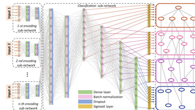
Fig. 2. DeeProtGO schematic representation. Several possible types of inputs are shown at the left, with their corresponding encoding sub-network. The middle part shows the classification model architecture, including the hierarchical layer architecture to model the outputs. The hierarchical structure of outputs are depicted at the right, indicated with different colors
