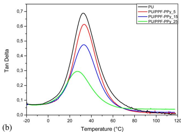
FIG. 6. DMTA traces (a) storage modulus and (b) loss factor of PU/PPF-PPy composites with various fillers contents. [Color figure can be viewed in the online issue, which is available at wileyonlinelibrary.com.]
