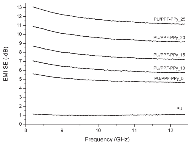
FIG. 8. EMI SE of PU/PPF-PPy composites with various fillers contents.
