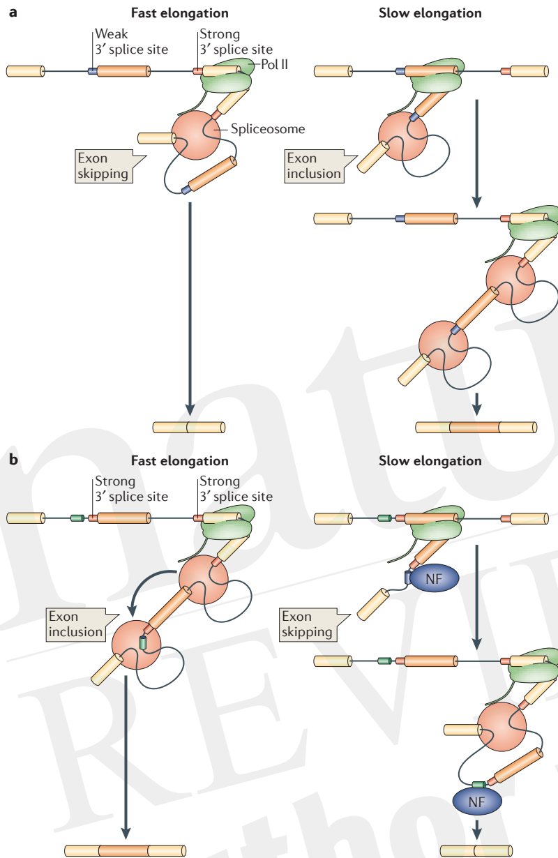
Figure 3 | Dual effects of transcriptional elongation on alternative splicing. a | During RNA polymerase II (Pol II)-mediated transcription, fast elongation (left) favours the recruitment of the spliceosome to the strong 3' splice site of a downstream intron instead of the weak 3' splice site of the upstream intron, which results in exon skipping. By contrast, slow elongation (right) favours the recruitment of spliceosome components to the upstream intron, which results in splicing commitment and exon inclusion. b | In conditions in which both 3' splice sites are equally strong and the upstream intron also has a binding site (green) for a splicing factor that inhibits exon inclusion (negative factor (NF)), fast elongation of Pol II (left) favours the recruitment of spliceosome components to both introns, ensuring exon definition and subsequent exon inclusion. On the contrary, slow elongation (right) provides a time window for the negative splicing factor to be recruited to its target site before spliceosome components can bind to the 5' splice site of the downstream intron and mediate exon definition. This results in exon skipping.
