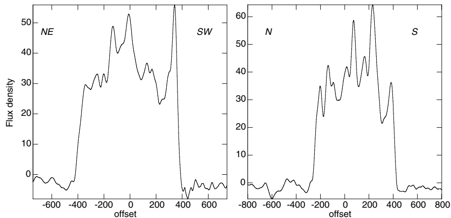
Figure 2. Two cuts across SNR G290.1–0.8 in the directions shown in Fig. 1 (NE–SW in the left-hand frame and N–S in the right). The flux density is given in mJy beam -1 , while the offsets are in arcsec and are referred to the central position in each cut.
