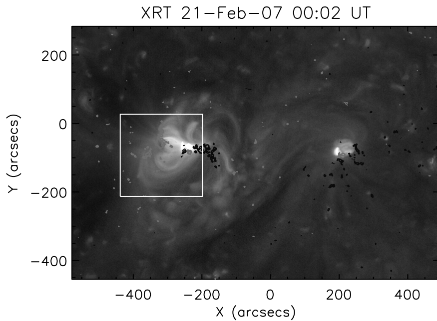
FIG. 3.—XRT image in the Ti\_poly filter with the MDI magnetogram shown in contours. The contour levels are 100 and 200 with white showing the positive magnetic field. The white box shows the EIS field of view.
