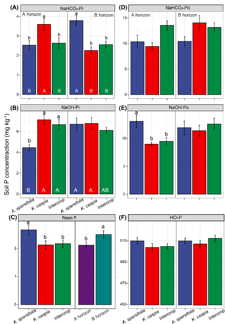
Figure 3. Concentrations of soil (A) NaHCO 3 -Pi, (B) NaOH-Pi, (C) Resin P, (D) NaHCO 3 -Po, (E) NaOH-Po, and (F) HCl-P in different soil horizons (A or B; depth) or different plant communities ( Alhagi sparsifolia (legume) monoculture, Karelinia caspia (non-legume) monoculture, or both species intercropped). Values are means \pm SE. Different capital letters below the bars indicate significant differences at p < 0.05 among six treatments, and lowercase letters above error bars indicate significant differences among different planting patterns and soil horizons at p < 0.05 .
