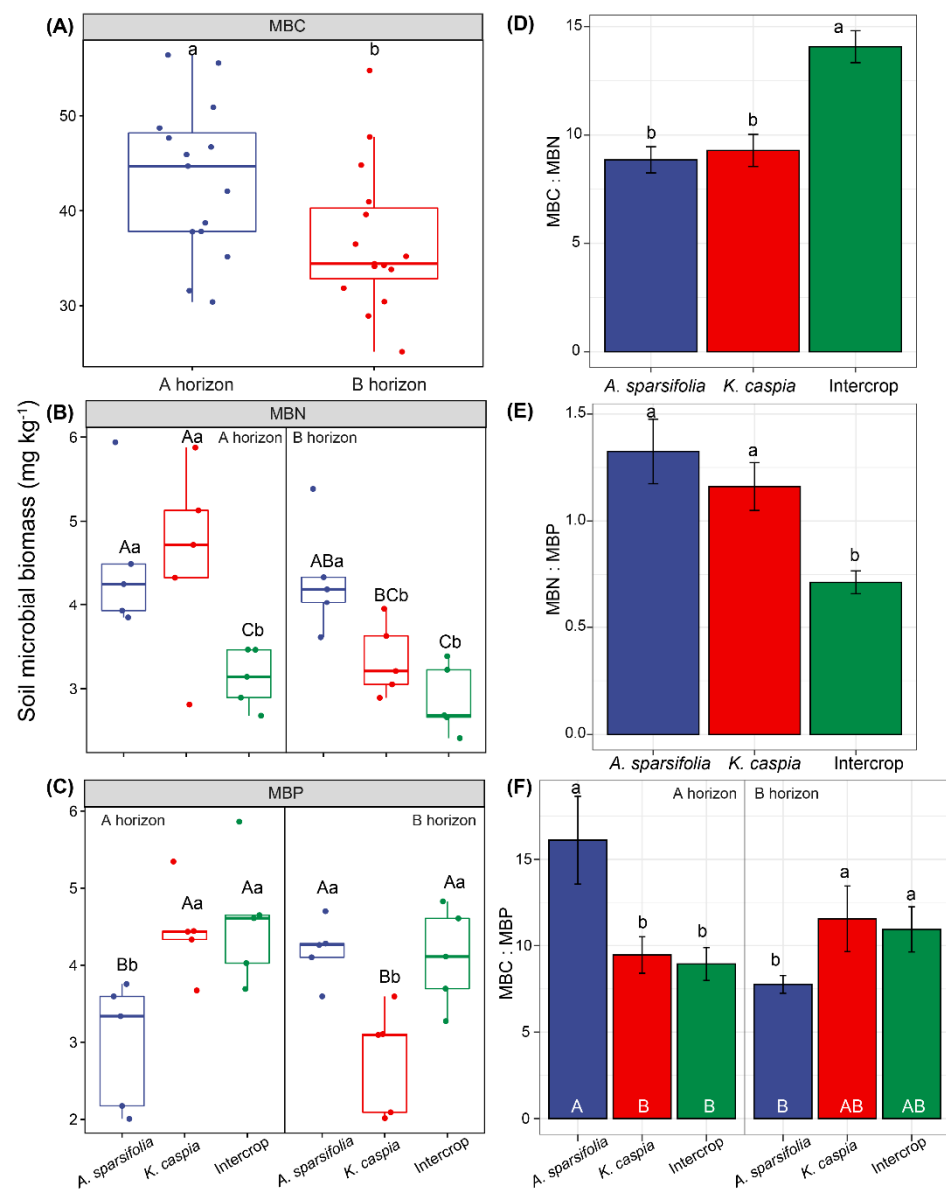
Figure 2. Effects of soil horizon (A or B; depth) and plant community ( Alhagi sparsifolia (legume) monoculture, Karelinia caspia (non-legume) monoculture, or both species intercropped) on (A) soil microbial biomass C (carbon), (B) microbial biomass N (nitrogen), (C) microbial biomass P (phosphorus), (D) microbial biomass C:N, (E) microbial biomass N:P, and (F) microbial biomass C:P. Values are means \pm SE. Different capital letters indicate significant differences at p < 0.05 among six treatments, and lowercase letters above error bars indicate significant differences at p < 0.05 among different plant communities and soil horizons, or among different plant communities within each soil layer.
