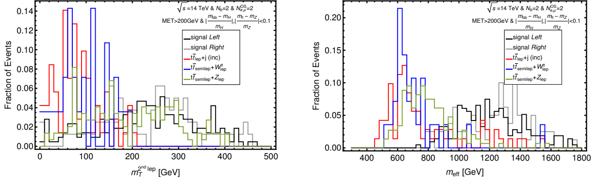
Figure 5. Distributions of the transverse mass of the second lepton m_T^{2nd lep} (left) and the effective mass m_{eff} (right), for signal and background after requiring two b -jets, two OS leptons and satisfying Equations (1)–(3).
