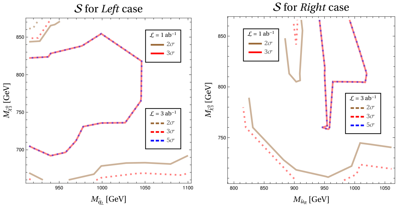
Figure 6. Contour lines in the plane [M_{\tilde{q}_L}, M_{\tilde{\chi}_3^0}] for \tilde{q}_L (left) and \tilde{u}_R (right) productions. Solid (dotted) lines correspond to \mathcal{L} = 1 ( 3 ) \text{ab}^{-1} . The brown, red and blue colors are the S (background systematic uncertainty of 30%) with values of 2\sigma , 3\sigma and 5\sigma , respectively.
