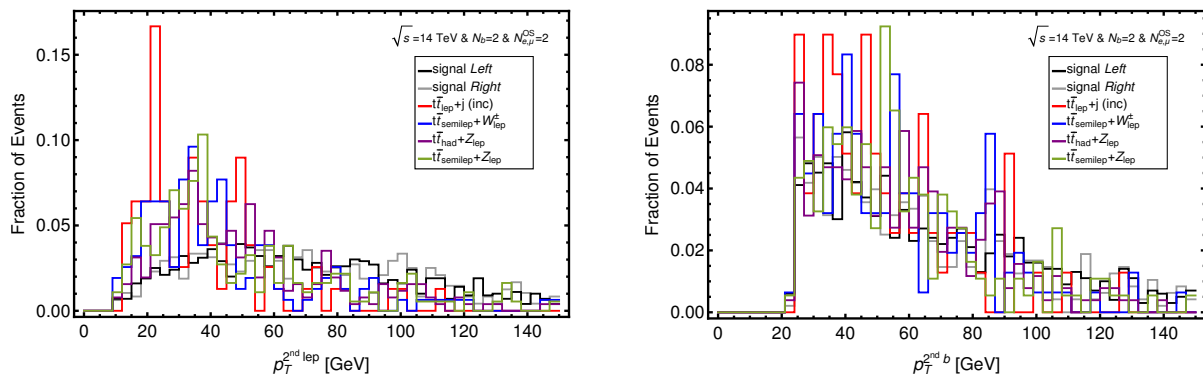
Figure 2. Distributions of transverse momentum of the second leading lepton p_T^{2nd lep} (left panel) and second leading b -jet p_T^{2nd b} (right panel) over samples of signal and backgrounds without parton-level cuts.
