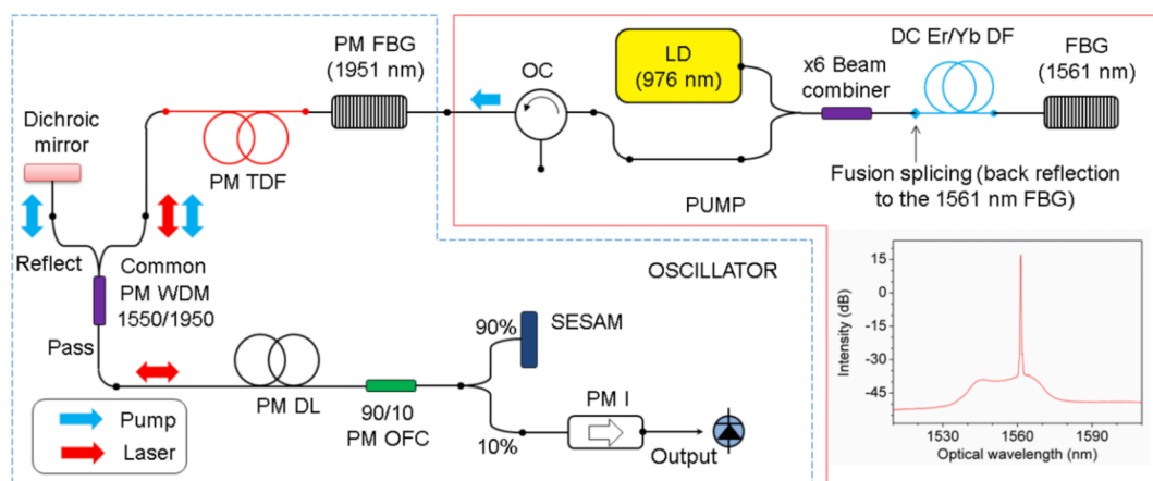
Fig. 1. The figure shows the experimental setup, with the solid lines enclosing the pump unit and the dashed lines enclosing the oscillator. The acronyms used stand for (starting from the top-right and following the different connections): Fiber Bragg Grating (FBG), dual-cladding Er/Yb doped fiber (DC Er/Yb DF), laser diode (LD), optical circulator (OC), polarization-maintaining fiber Bragg grating (PM FBG), polarization-maintaining thulium doped fiber (PM TDF), polarization-maintaining wavelength division multiplexer (PM WDM), polarization-maintaining delay line (PM DL), polarization-maintaining optical fiber coupler (PM OFC), semiconductor saturable absorber mirror (SESAM), and polarization-maintaining isolator (PM I). In addition the spectrum at the output of the CW pump is shown; see the inset in the pump block.
