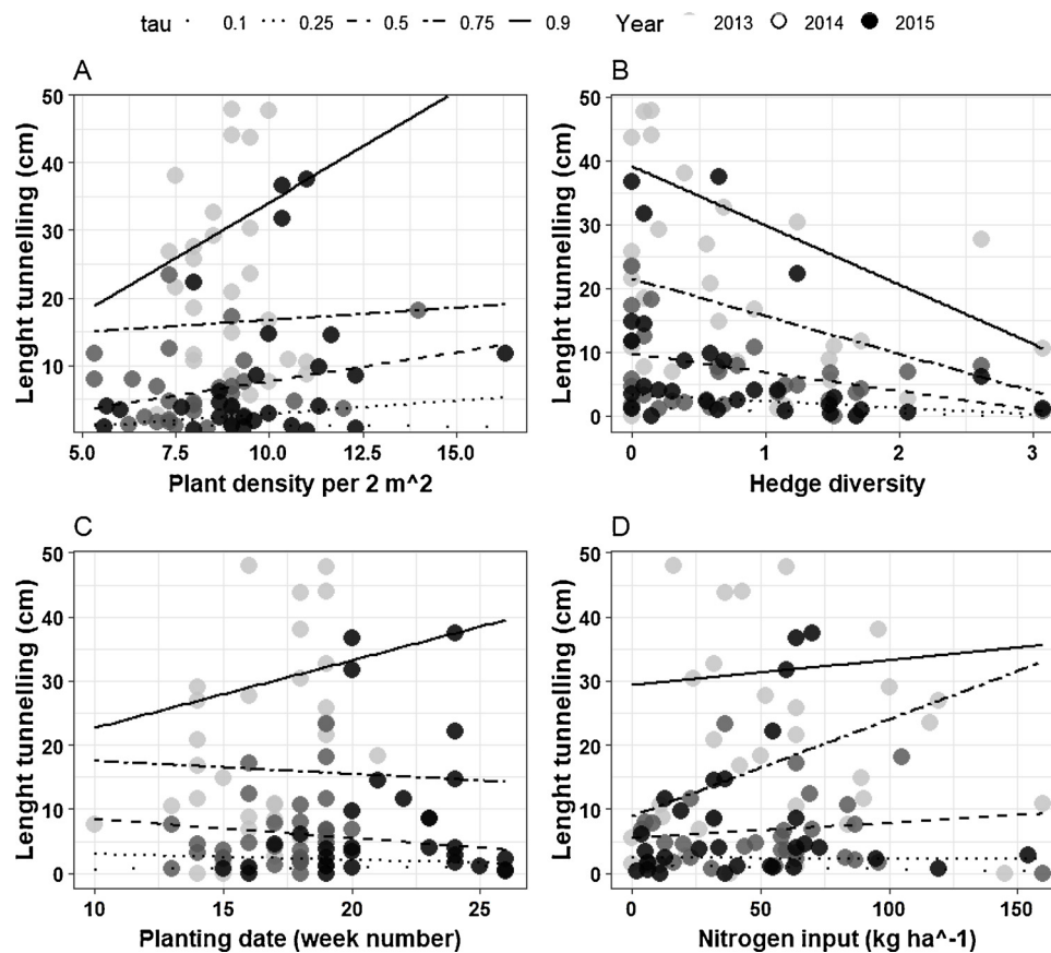
Fig. 3. Quantile regressions at 10, 25, 50, 75 and 90% of the length tunnelling for the field scale variables plant density (A), hedge diversity (B), planting date (C) and nitrogen input (D).
