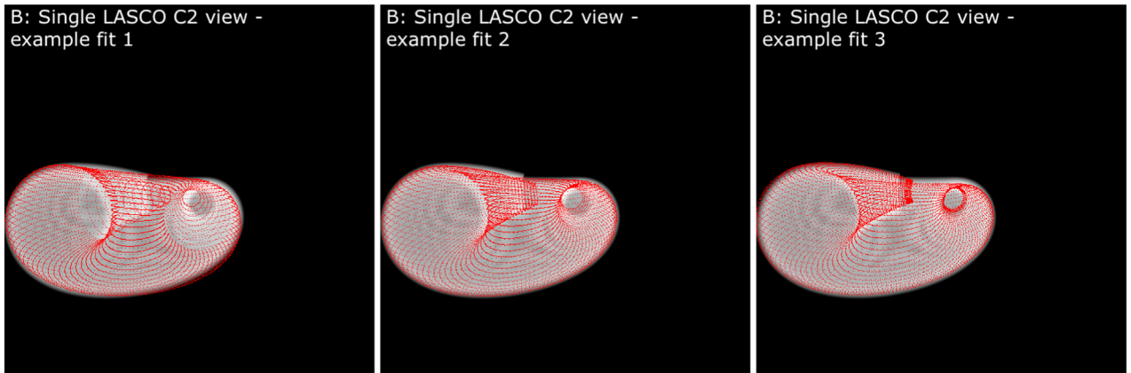
Fig. 4. Examples of different fits to LASCOS synthetic images using only one viewpoint from configuration B (L5-like), performed by three different observers. These examples illustrate a wide range in values for the half-angle. All three fits visually appear equally valid, however, they correspond to half-angles of 29°, 48°, and 63°, and to latitudes of -6°, -10°, and -11° from left to right, demonstrating the projection effects.
