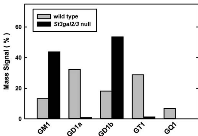
Fig. 5. Quantification of MS peak intensities of permethylated gangliosides from wild-type and St3gal2/3 -double-null mice.
