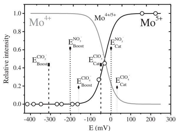
Fig. 6. EPR titration; variation of the Mo V signal intensity (empty circles) with potential (vs. SHE). Black solid line is the Nernstian fit of the experimental data assuming E_{im}^{(V/IV)} = -30 mV. Measurements conditions: microwave frequency, 9.65 GHz; temperature, 25 K; microwave power, 0.6 mW; modulation frequency, 10 kHz; modulation amplitude, 5 Gpp; buffer, 10 mM Tris-HCl pH 7.60.
