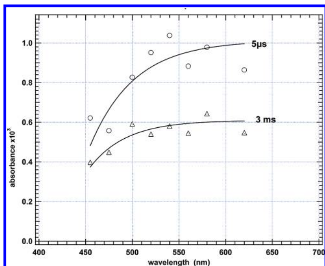
Figure 8. Transient absorption spectra of D-TKP 102-A powder.
