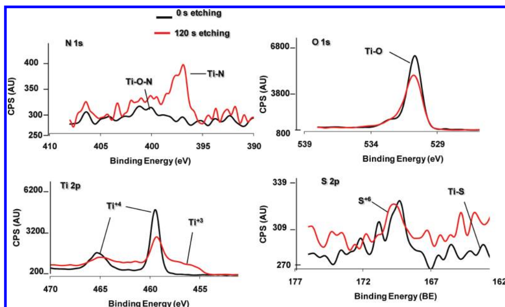
Figure 5. XPS \text{Ar}^+ sputtering measurements (etching time of 120 s) of D-TKP 102-A powder.
