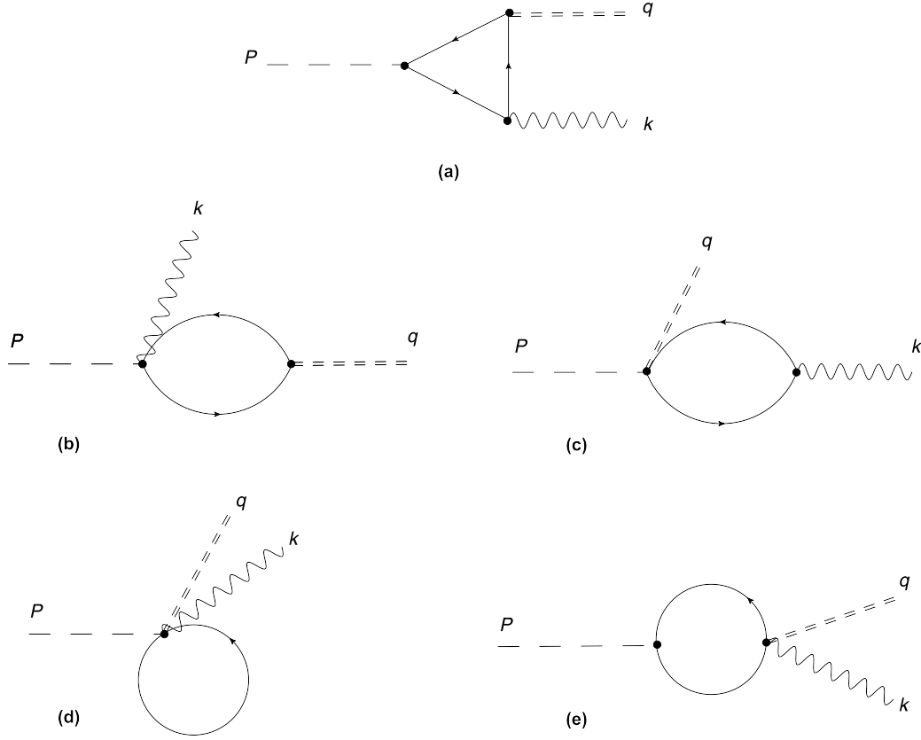
Fig. 1. Diagrammatic representation of the possible contributions to \pi^+ \rightarrow e^+ \nu_e \gamma decay. Double-dashed lines, wavy lines and single-dashed lines represent the e\nu_e pair, the outgoing photon and the decaying pion, respectively. While for the vector form factor only the contribution from the triangle diagram (a) is nonvanishing, in the case of the axial-vector form factor all five diagrams contribute.
