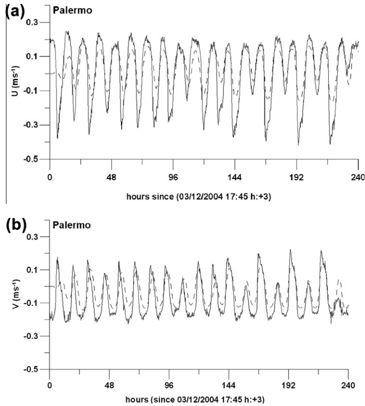
Fig. 7. Observed (solid) and simulated (dashed) east–west (a) and north–south (b) current components at Palermo ( \text{ms}^{-1} ).
