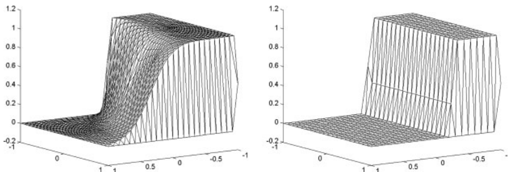
FIG. 4. Left: Test 2 with \beta = [2/3, 2] and an unstructured mesh; Right: Test 2 with \beta = [0, 1] and a mesh aligned to the transport direction.
