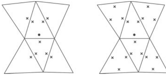
FIG. 2. Left: Connectivity for modified LDG (left) standard LDG (right).
