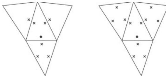
FIG. 1. Connectivity for modified IP (left) and standard IP (right).
