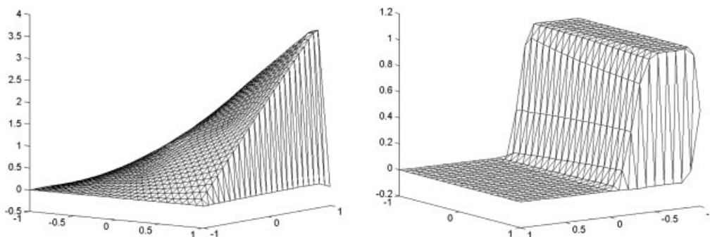
FIG. 7. Tests described in Remark 5.1.
