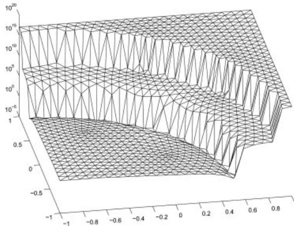
FIG. 5. Test 3, in semilogarithmic scale.
