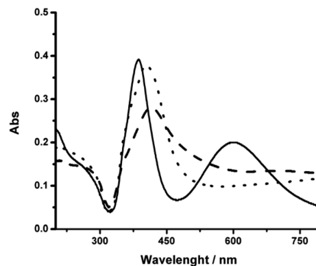
Fig. 2 UV-vis spectra of nanosilver colloidal dispersions after synthesis at different NaOH concentrations (mM): 1 (—), 1.8 (---) and 3 (- · -). The spectra were measured after centrifugation and resuspension in water at 25.0 °C.
