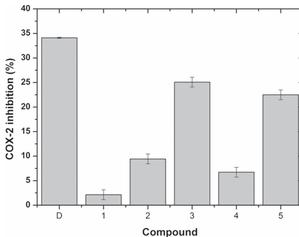
Figure 4. Anti-inflammatory activity of FA and its derivatives, measured as inhibition of COX-2 in vitro . Concentrations tested: Diclofenac (D), 0.1 M; FA and its mono- and diesters, 1.0 M.
