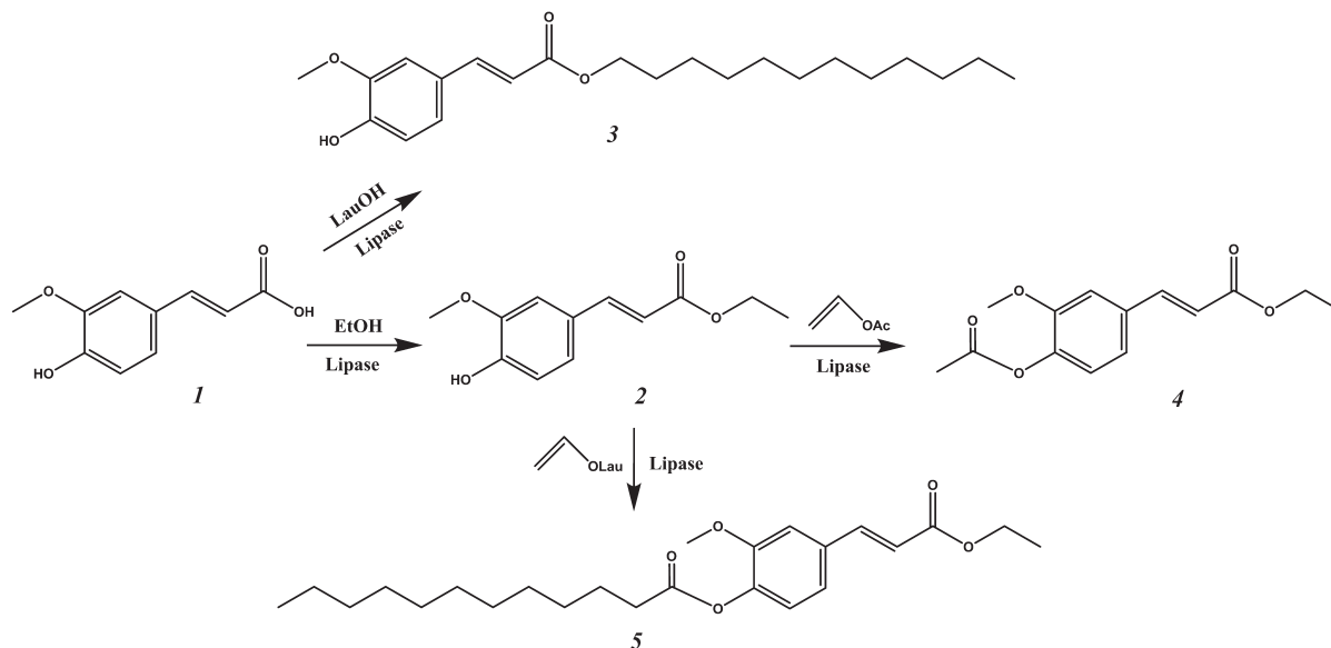
Figure 1. Scheme of the lipase-catalyzed synthesis of FA mono- and diesters.
