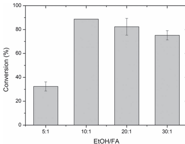
Figure 2. Effect of ethanol/FA molar ratio on CALB-catalyzed synthesis of EF. Reaction conditions: 10 mg/mL FA; Solvent: diisopropyl ether (DIPE); 100 mg/mL biocatalyst (CALB); Temperature 60°C; Reaction time: 7 days. Conversion was determined by HPLC.
