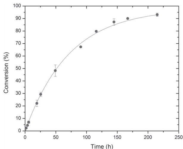
Figure 3. Time course of EF synthesis in DIPE catalyzed by CALB. Reaction conditions: 10 mg/mL FA; 100 mg/mL biocatalyst; Temperature 60°C. Conversion was determined by HPLC.
