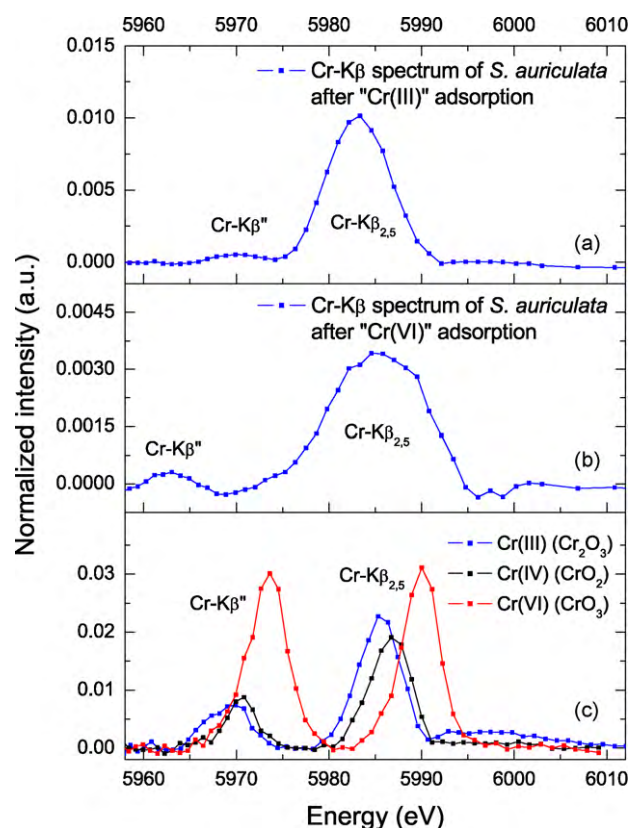
Fig. 4. Comparison between the partial Kβ spectra in the energy region of Kβ 2,5 of Salvinia auriculata samples after the Cr adsorption processes of (a) trivalent, (b) hexavalent Cr solutions, and (c) Cr-Kβ spectra of reference materials.
