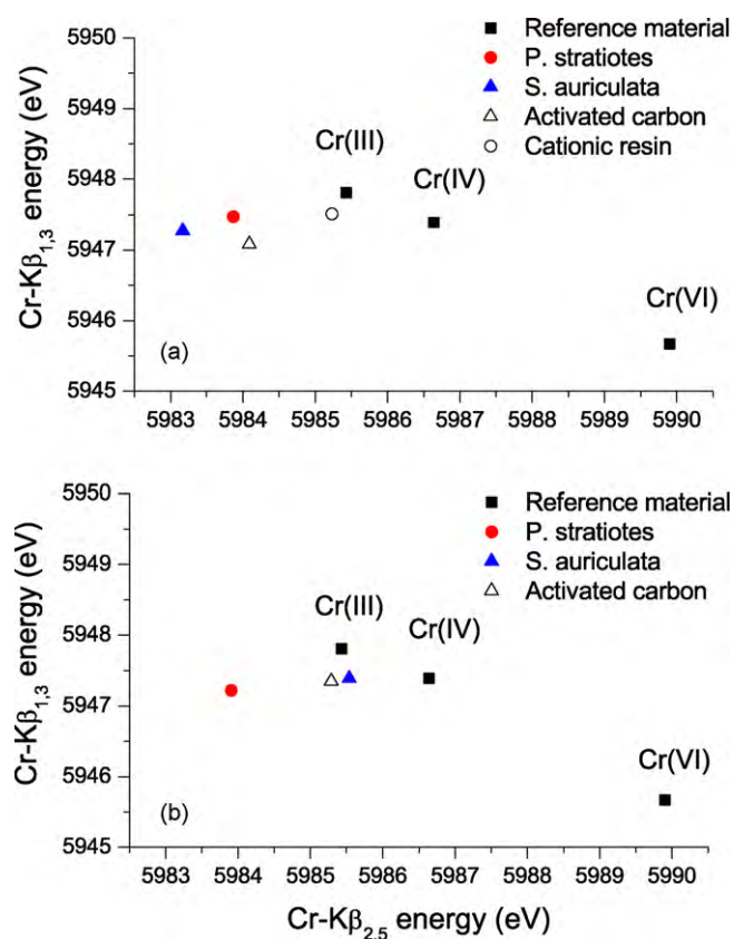
Fig. 7. Comparison between Cr-K \beta_{1,3} energy as function of Cr-K \beta_{2,5} energy of Cr reference materials, Pistia stratiotes , Salvinia auriculata , activated carbon, and cationic-exchange resin samples after the Cr adsorption processes of (a) trivalent and (b) hexavalent Cr solutions.
