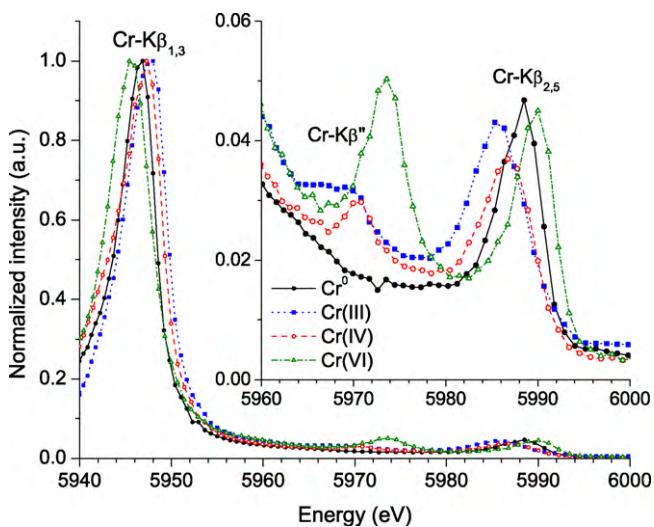
Fig. 1. Cr-K \beta spectra for metallic Cr and Cr compounds (Cr 2 O 3 , CrO 2 , and CrO 3 ). Black (solid), blue (dot), red (dash), and green (dash-dot) lines correspond to Cr 0 , Cr(III), Cr(IV), and Cr(VI), respectively.
