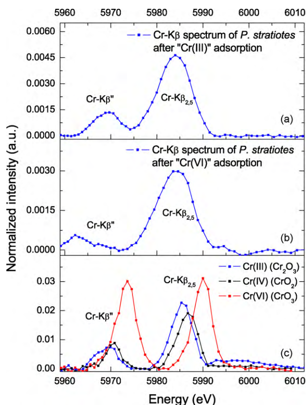
Fig. 3. Comparison between the partial Kβ spectra in the energy region of Kβ 2,5 of Pistia stratiotes samples after the Cr adsorption processes of (a) trivalent, (b) hexavalent Cr solutions, and (c) Cr-Kβ spectra of reference materials.
