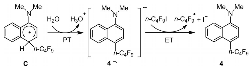
Scheme 8. Possible reaction mechanism involving a radical anion species.
