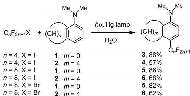
Scheme 3. Perfluoroalkyl group substitution of aromatic amines in water.
