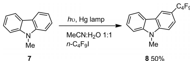
Scheme 4. Photoinduced perfluorobutylation reaction of carbazole rings in MeCN/H 2 O.
