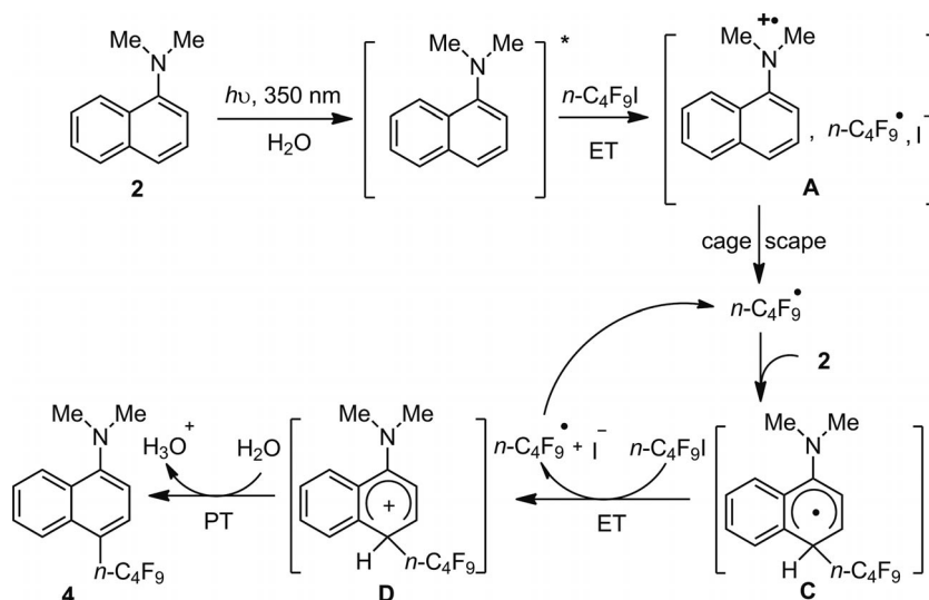
Scheme 7. Proposed reaction mechanism for the photoinduced ET (PET) perfluorobutylation substitution of aromatic amines in water.
