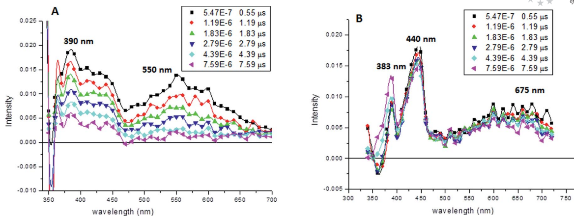
Figure 2. Transient UV/Vis spectra of N,N -dimethyl-1-naphthylamine 2 ( 0.8 \text{ mmol dm}^{-3} in MeCN) after 0.55, 1.2, 1.8, 2.8, 4.4, and 7.6 \mu\text{s} of laser pulsing at 355 nm excitation wavelength: (A) in the absence of n -C 4 F 9 I; (B) in the presence of n -C 4 F 9 I ( 11.6 \text{ mmol dm}^{-3} ).
