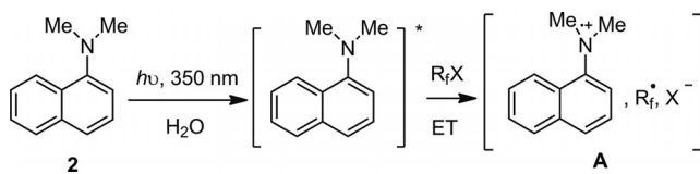
Scheme 6. PET between 2 and R f X to generate radical ion pair A.
