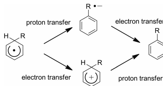
Scheme 1. PT and ET of cyclohexadienyl-type radicals.
