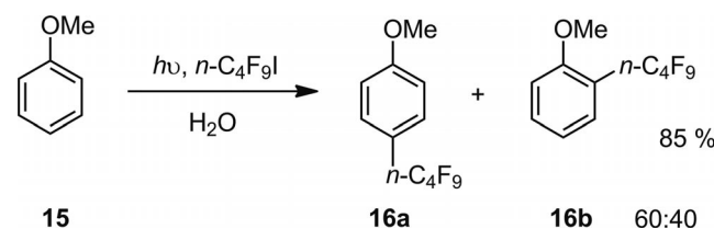
Scheme 5. Perfluorobutyl group substitution of anisole in water.
