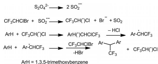
Scheme 2. Mechanism for the aromatic radical substitution reaction of H for R f . [7]
