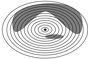
Figure 2: Schematic drawing of the inverse mean curvature flow from a typical point. The last surface is defined as the first one that enclosed the domain U .
