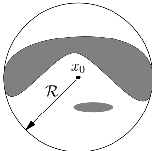
Figure 1: The domain U is colored with gray. The radius \mathcal{R} is defined as the radius of the smallest sphere that encloses U . For this particular domain U the center x_0 of that sphere is not in U .
