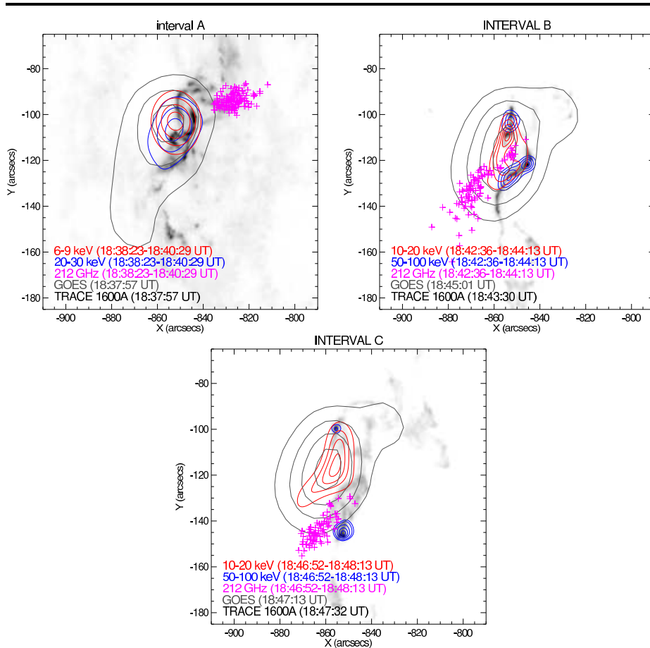
Figure 6. RHESSI hard X-ray (thermal emission in red and non-thermal in blue contours), GOES soft X-ray (thin black contours), and TRACE UV images background continuum gray-black areas during phase (A), (B), and (C) (see Figure 1). 212 GHz centroid positions (same as in Figure 5) are shown as magenta crosses for comparison.
