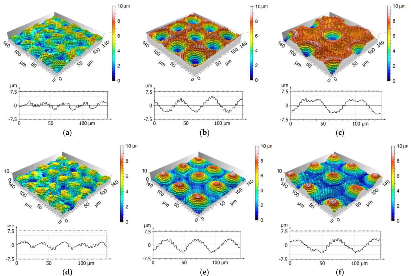
Figure 9. Confocal images and extracted profiles of hierarchical microstructures on stainless steel (a–c) and a hot embossed PET foil (d–f). Distance between spots was (a,d) 30\ \mu\text{m} , (b,e) 50\ \mu\text{m} , and (c,f) 70\ \mu\text{m} . Profiles were extracted with a length of 140\ \mu\text{m} at a range of 15\ \mu\text{m} .
