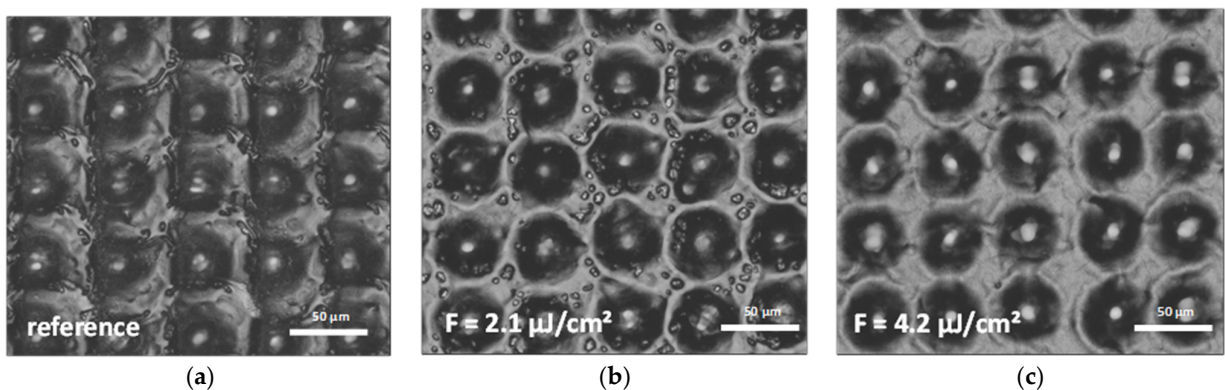
Figure 5. (a) Optical microscopy images of a stainless steel surface patterned with DLW with a spot distance of 60 \mu\text{m} using 500 laser pulses at a pulse duration of 200 ns and a fluence of 0.44 \text{J}/\text{cm}^2 . (b) Patterned surface with an additional laser polish step at a fluence of 2.1 \mu\text{J}/\text{cm}^2 and (c) 4.2 \mu\text{J}/\text{cm}^2 .
