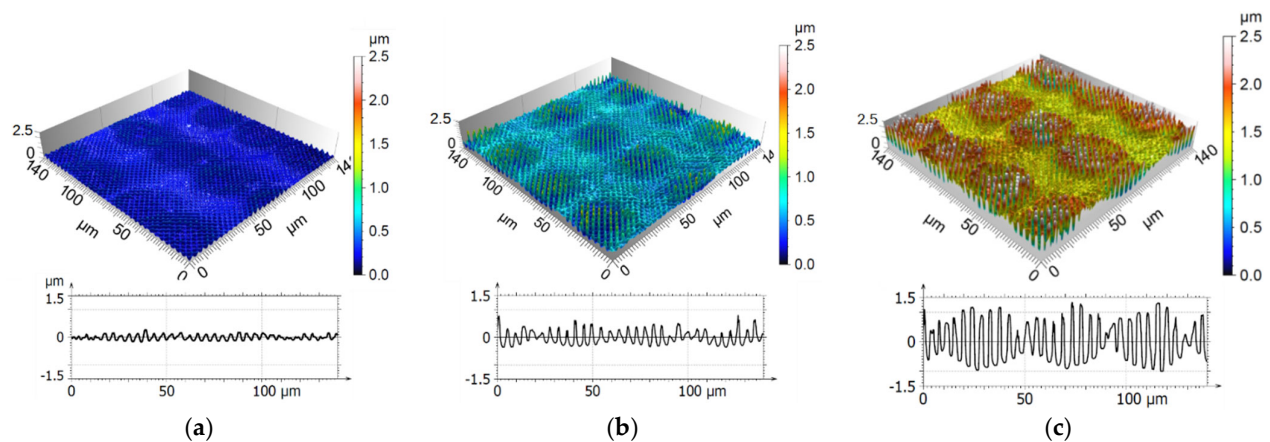
Figure 7. Confocal microscopy images of periodic microstructures and extracted profiles of DLIP structured stainless steel surfaces with (a) 1, (b) 5, and (c) 10 applied pulses. The measured average structure depth was (a) 0.23 \mu\text{m} , (b) 0.74 \mu\text{m} , and (c) 1.74 \mu\text{m} .
