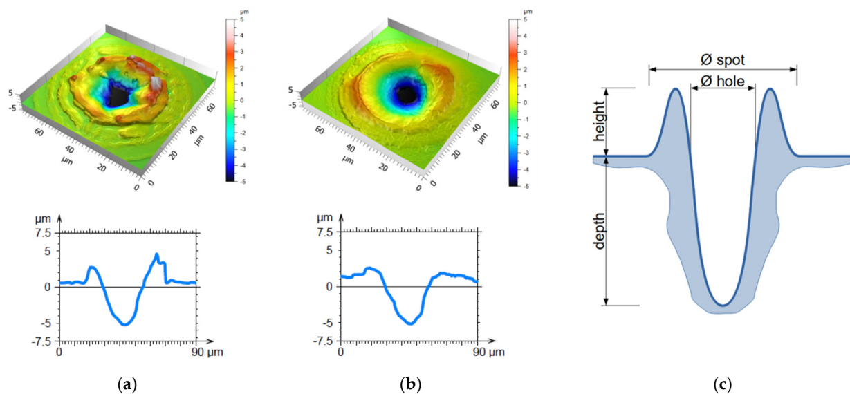
Figure 3. Confocal images and profiles of spots processed with DLW using (a) 70 pulses with a pulse duration of 8 ns and (b) 400 pulses at 200 ns. The laser fluence was kept constant at of 0.44 J/cm 2 . The resulting holes had a depth of approximately 5.0 \mu\text{m} in both cases. (c) Schematical drawing of the cross section of a laser processed spot defining the structure depth, height of molten material, and spot and hole diameters.
