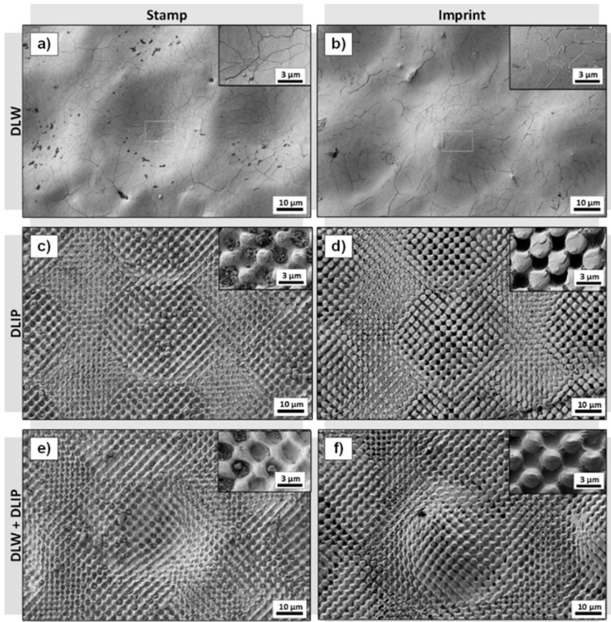
Figure 8. Scanning electron images of laser processed surfaces on stainless steel using (a) DLW technique, (c) DLIP technique, and (e) combined DLW and DLIP techniques. Surface structures were transferred to PET foil (b,d,f) using plate-to-plate-hot embossing. DLW structures were processed, using a 1064 nm pulse laser system, operating at 30 kHz and a pulse length of 200 ns. Spot distance was set to 70 \mu\text{m} . For DLIP, 10 pulses with constant fluence of 0.17 \text{mJ}/\text{cm}^2 were applied.
