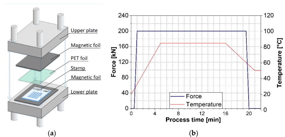
Figure 2. (a) Schematics of plate-to-plate hot embossing. (b) Applied forced and temperature as a function of process time for hot embossing experiments, performed within this study.
