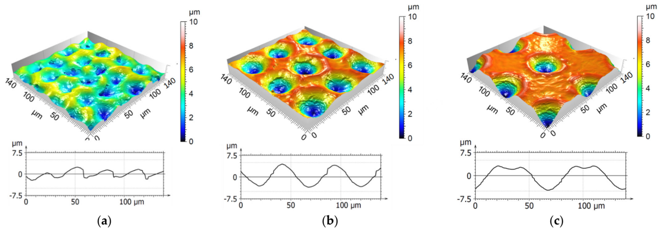
Figure 6. Confocal images and corresponding profiles of stainless steel surfaces micropatterned with 500 pulses with a pulse duration of 200 ns and a fluence of 0.44 J/cm 2 . The DLW spot distance was set to (a) 30 \mu\text{m} , (b) 50 \mu\text{m} , and (c) 70 \mu\text{m} .
