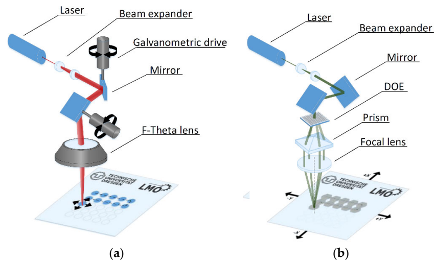
Figure 1. Schematics of (a) direct laser writing (DLW) and (b) direct laser interference patterning (DLIP). The DLW system operated at 1064 nm with pulse durations of 8 ns, 50 ns or 200 ns. For the DLIP technique, a laser beam was split with a diffractive optical element and recombined by a lens. The interference pattern was guided over the surface using 2 linear stages. Overlapping 4 beams lead to interference in the focal volume, resulting in an intensity with a dot-like distribution. Moving the target in X and Y directions with high precision linear stages, large areas can be structured.
