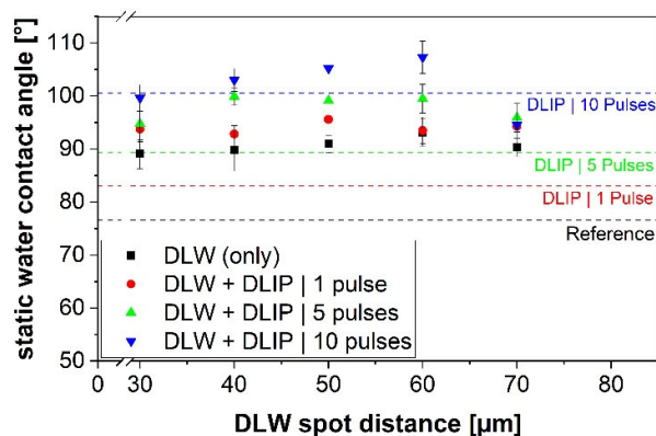
Figure 10. Measured static water contact angle on PET foils imprinted with different single- and multi-scale structures. Multi-scale structures were processed combining the DLW and DLIP techniques. Single-scaled DLW structures are shown as black values, whereas single-scaled DLIP structures are represented with dashed lines. Error bars indicates the mean value of 5 measurements. Black dashed line represents the reference on a flat PET surface.
