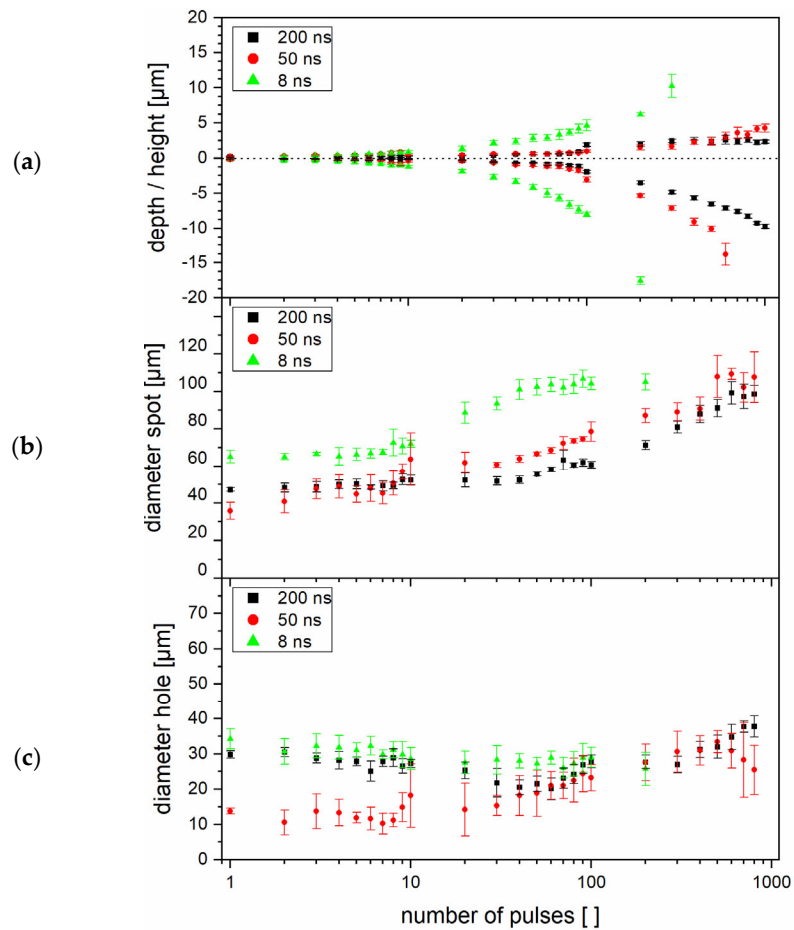
Figure 4. (a) Measured structure depth and height relative to the untreated surface, (b) spot diameter and (c) hole diameter for DLW processed holes on stainless steel according to the definition in Figure 3c. The error bars represent the standard deviation of 8 measured spots.
