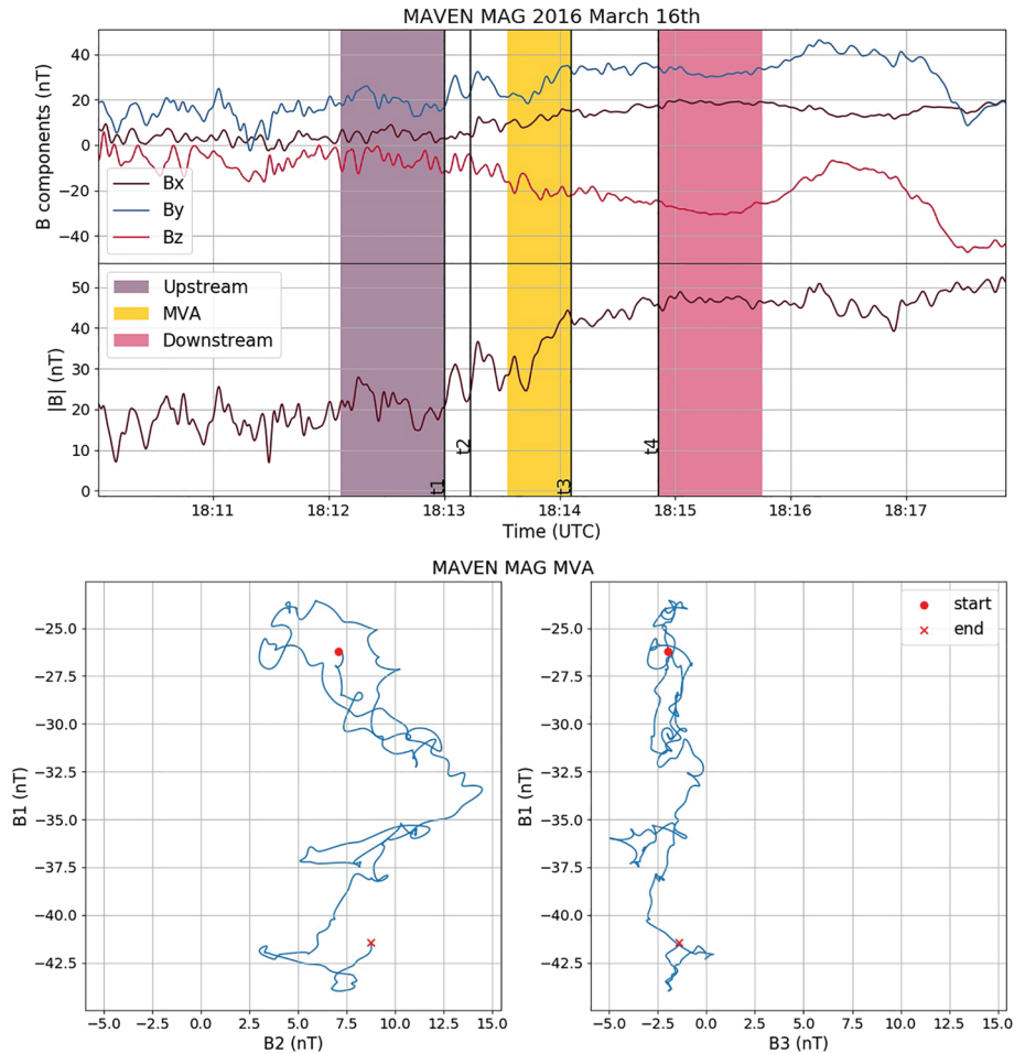
Figure 2. Magnetic field components in MVA coordinates and amplitude (top). The upstream and downstream intervals from the MPB and the interval where MVA was applied are shaded. Magnetic hodograms ( N = 922 , \lambda_2/\lambda_3 = 9.8 ) depicting the magnetic field projection on the planes (\hat{e}_1, \hat{e}_2) and (\hat{e}_1, \hat{e}_3) in the interval where MVA was applied (bottom). The start point is marked with a circle and the end point with a cross.
