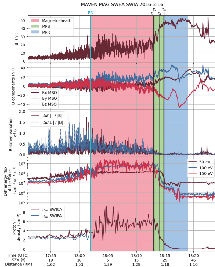
Figure 1. Time series of the magnetic field and plasma data from MAVEN for the 16 March 2016 crossing. (from top to bottom) Magnetic field magnitude, magnetic field components, relative variation of the magnetic field, differential energy fluxes for solar wind electrons, and solar wind proton density. The MPB is shaded in green, the magnetosheath in red, and the MPR in blue.
