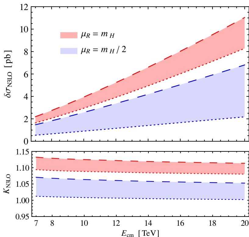
Figure 4. The N 3 LO contribution to the Higgs production cross section as a function of the collider energy for the SV approximation (dotted) and the SV terms plus the \mathcal{O}(N^{-1}) contributions in eq. (3.3) (dashed) at \mu_R = m_H (upper curves) and \mu_R = 0.5 m_H (lower curves) for the NNLO gluon distribution of ref. [53] at \mu_F = m_H . The lower panel shows the ratio of these N 3 LO predictions to the complete NNLO result.
