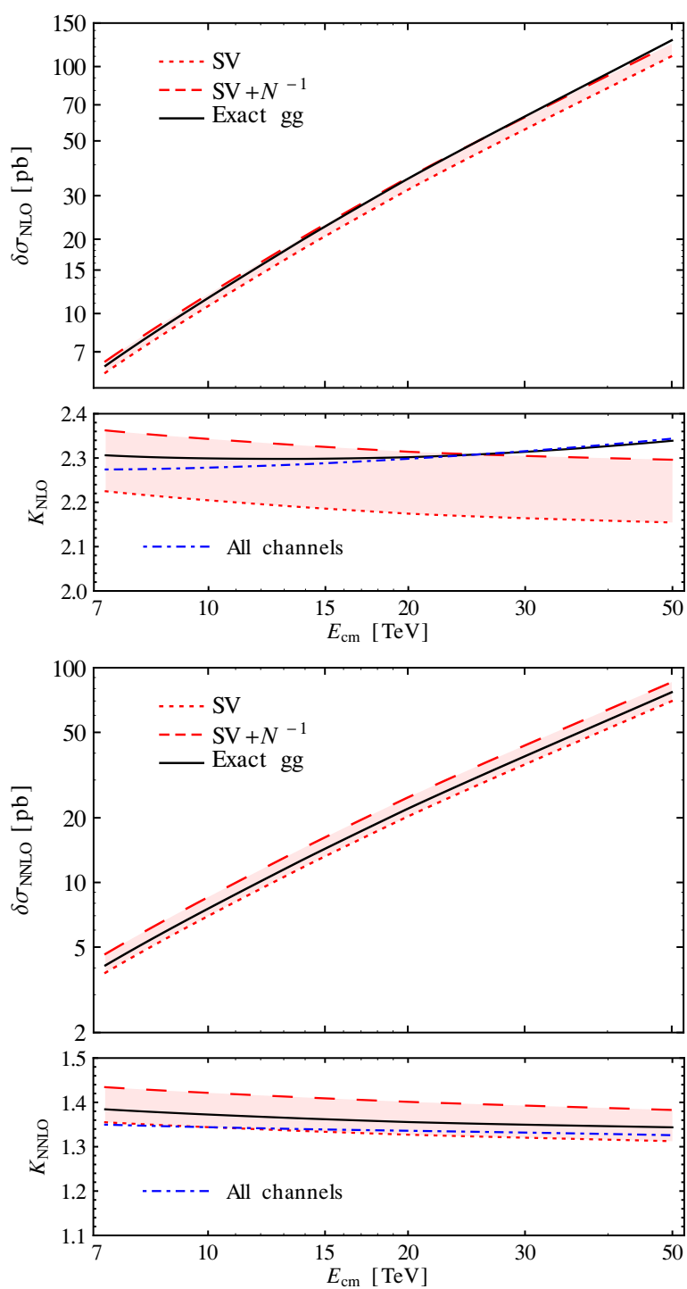
Figure 3. The NLO (top) and NNLO (bottom) gluon-gluon contributions to the Higgs production cross section as a function of the collider energy for the exact coefficient function (solid), the SV approximation (dotted) and the SV terms plus the N^{-1} contributions (dashed). The lower panels show the corresponding K -factors, including the impact of the other partonic subprocesses (dash-dotted). All curves have been calculated using the central NNLO \alpha_s and parton densities of ref. [53].
