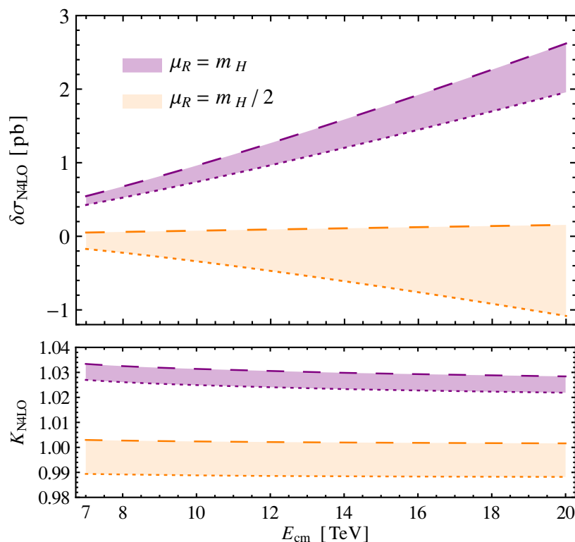
Figure 6. As figure 4, but for the N 4 LO corrections as obtained from the ‘large’ and ‘small’ SV estimates of the coefficient function c_{gg}^{(4)}(N) discussed in the text. In the lower panel the N 4 LO results are shown relative to the corresponding N 3 LO cross sections in the SV approximation.
