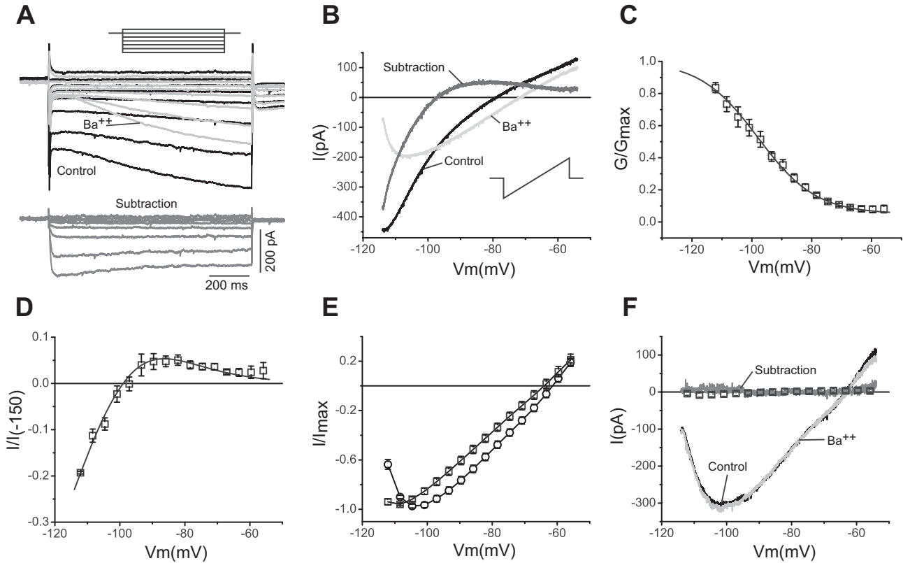
Fig. 1. Characterization of a strong inward rectifier potassium current ( I_{Kir} ) in thalamocortical (TC) neurons. A : voltage-clamp recordings before (black traces) and after (light gray traces) application of 50 \mu\text{M Ba}^{2+} (top). Bottom traces (dark gray) show the barium-sensitive component obtained by subtraction. The recordings were obtained using a protocol of square pulses from -124 to -64 mV in increments of 10 mV (inset) from a holding potential of -74 mV. B : barium experiment similar to that in A using a slow ramp from -114 to -54 mV (inset). Conventions as in A ; V_m , membrane potential. C : normalized barium-sensitive conductance ( G/G_{\text{max}} ) from 8 cells (average \pm SE) obtained using the ramp protocol in B , with superimposed average Boltzmann fit (solid line). D : barium-sensitive current obtained with the ramp protocol from 8 cells (average \pm SE) normalized to the extrapolated current at -150 mV ( I/I_{-150} ; see METHODS). Superimposed (solid line) is the simulated current-voltage ( I - V ) curve obtained with a model using the parameters of the Boltzmann fit from C and \bar{g}_{Kir} (average maximum conductance) = 2.0 \times 10^{-5} S/cm ^2 . E : normalized current ( I/I_{\text{max}} ; average \pm SE) from wild-type ( \square ; n = 24 ) and Kir2.2 knockout (KO) mouse TC neurons ( \circ ; n = 19 ) obtained with the ramp protocol in the absence of pharmacological agents. F : voltage-clamp recordings before and after application of 50 \mu\text{M Ba}^{2+} and barium-sensitive component obtained by subtraction from a Kir2.2 KO TC neuron. Conventions as in A and B . Superimposed ( \square ) is the average \pm SE (error bars are not visible) barium-sensitive component from 8 cells.
