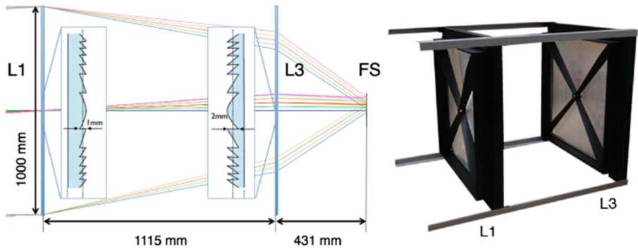
Fig. 5 Left: raytracing diagram for the EUSO-Balloon optics with the Fresnel Lenses L1 and L3, and the focal surface FS; the incident rays are at off-axis angles ranging from 0° (blue) to 1° (green), 2° (red) 3° (yellow) and 4° (purple); inserts show partial sectional views of L1 and L3; right: the Fresnel lenses L1 and L3 (8 mm thick PMMA, surface of 1 × 1 m 2 ) mounted onto their fiberglass frames and spiders, and held at a distance of 1.11 m by an optical “sled”
