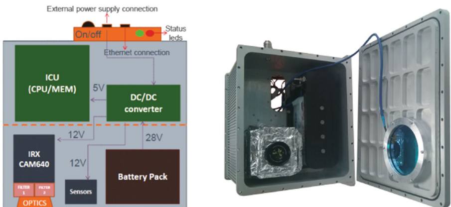
Fig. 6 Left: block diagram of the stand-alone IRcam system; right: the rugged watertight aluminium housing (0.4 × 0.4 × 0.4 m) of the IRcam with the IRX CAM640 in its lower left side
