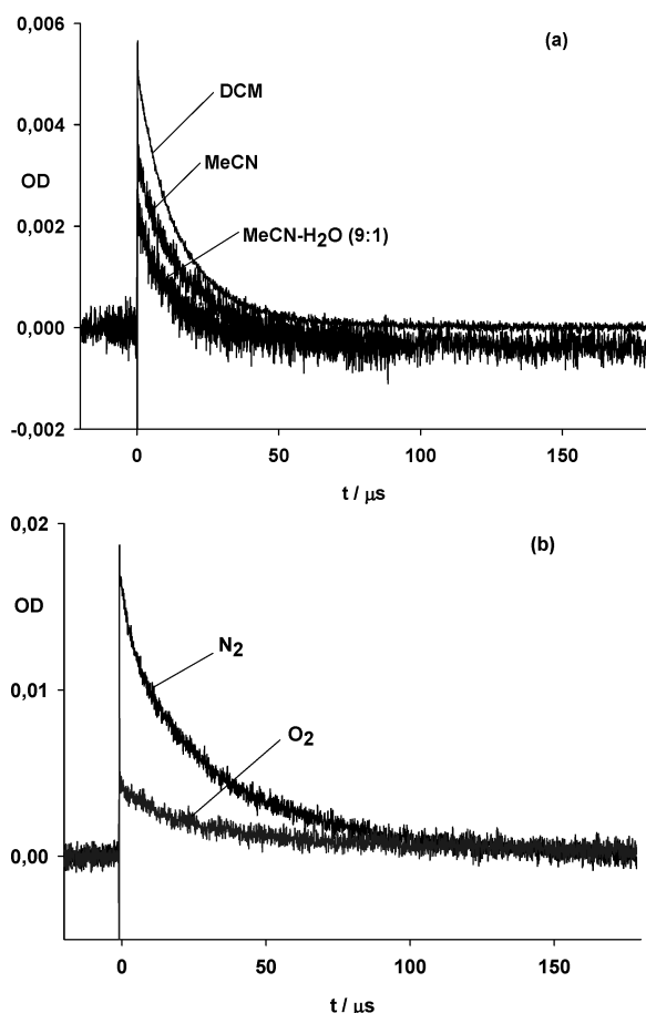
Figure 3. (a) Decay traces of \text{PPh}_3^+ after a laser pulse ( \lambda_{\text{exc}} : 355 nm) of \text{N}_2 -saturated solutions of \text{PPh}_3 ( 0.010 \text{ mol}\cdot\text{dm}^{-3} ) and NMQ ( 1.0 \times 10^{-4} \text{ mol}\cdot\text{dm}^{-3} ) in dichloromethane, MeCN, and MeCN- \text{H}_2\text{O} 9:1 mixture recorded at 510 nm. (b) Decay traces of \text{PPh}_3^+ after a laser pulse ( \lambda_{\text{exc}} : 355 nm) of \text{N}_2 - and \text{O}_2 -saturated acetonitrile solutions of \text{PPh}_3 ( 0.010 \text{ mol}\cdot\text{dm}^{-3} ) and S-TTP ( 1.0 \times 10^{-4} \text{ mol}\cdot\text{dm}^{-3} ) recorded at 510 nm.
