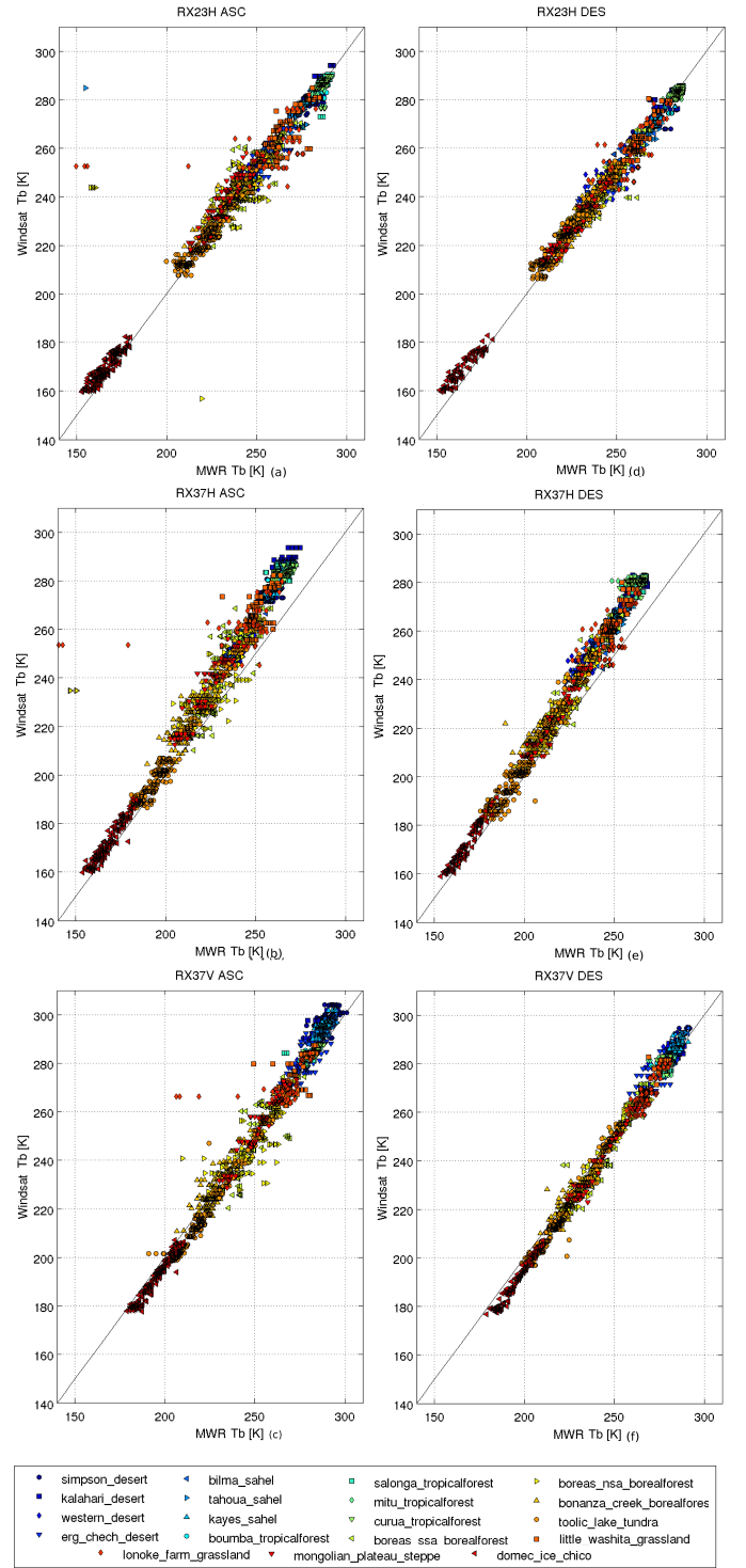
Fig. 6. Cross calibration of Tb23H, Tb37H and Tb37V for ASC and DESC passes.
