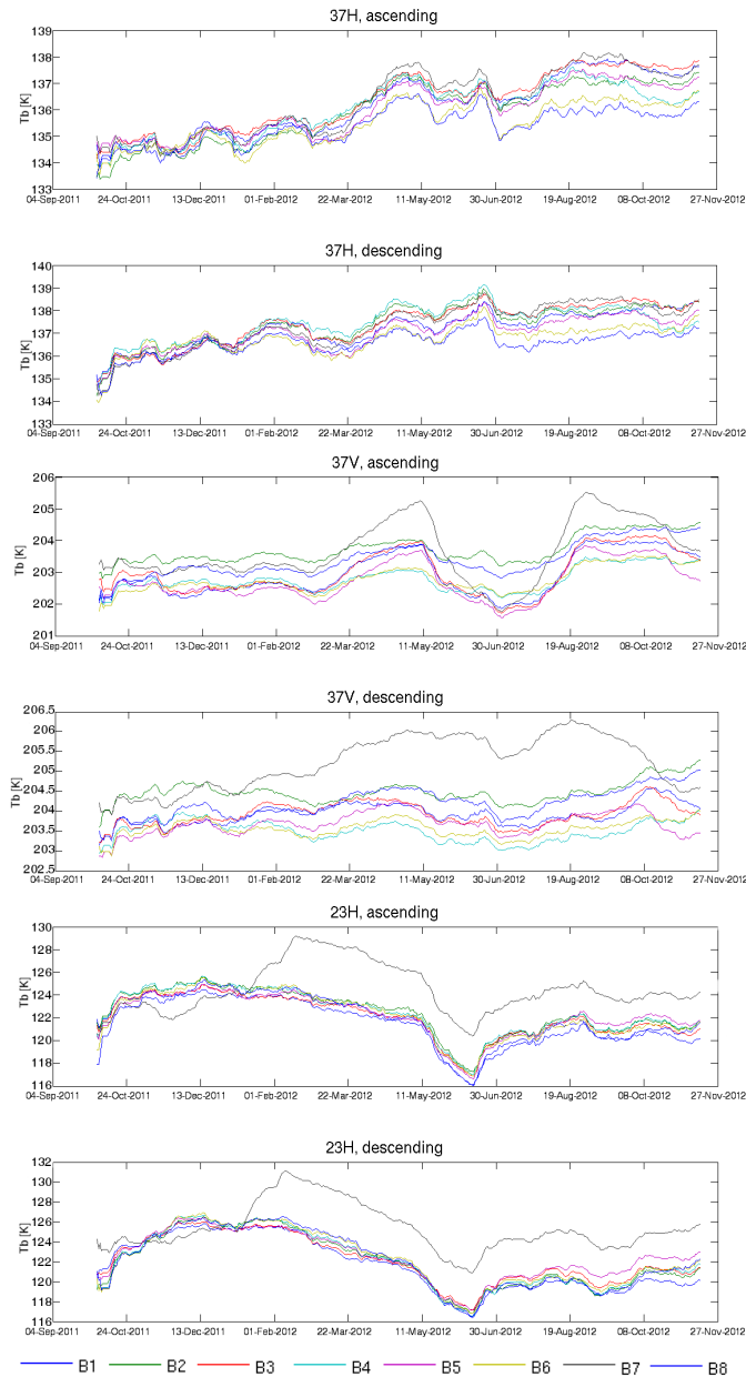
Fig. 4. Time Series of Vicarious Cold Values
