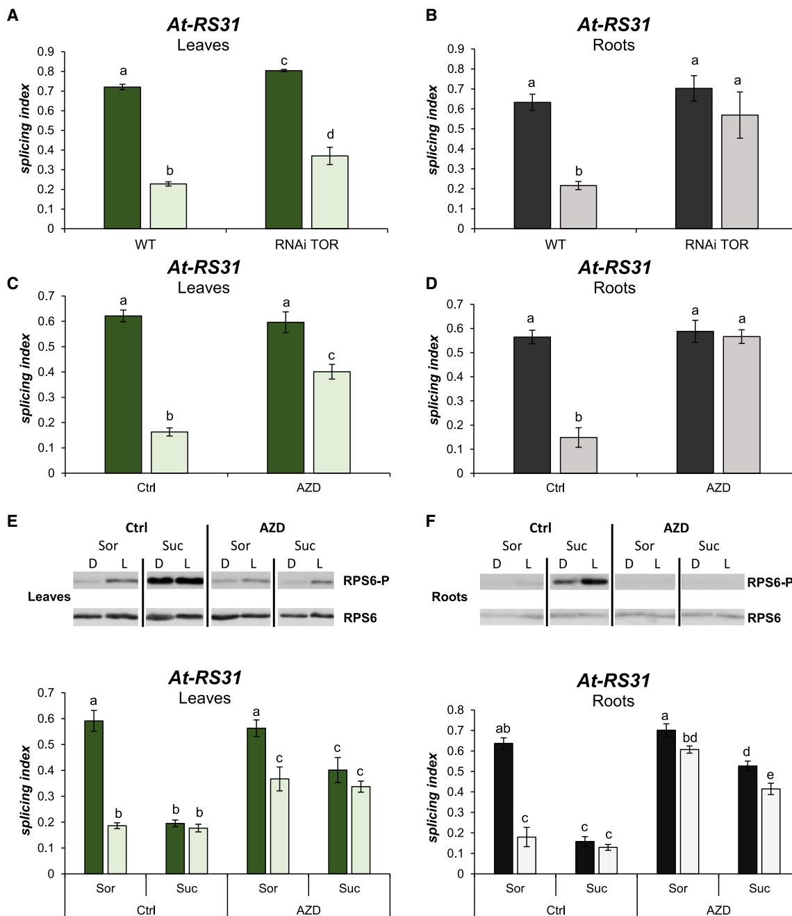
Figure 2. TOR kinase modulates alternative splicing responses to light and sugars in roots
