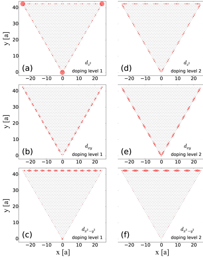
FIG. 2. Square magnitude of wave function components, as indicated by the radius of red circles, for two in-gap levels: (a)–(c) level 1 ( \epsilon_{F1} = 0.9305 eV) and orbitals (a) d_{z^2} , (b) d_{xy} , and (c) d_{x^2-y^2} ; (d)–(f) level 2 ( \epsilon_{F2} = 0.7688 eV) and orbitals as shown. Black dots indicate Mo sites. The d_{xy} and d_{x^2-y^2} components have been amplified by a factor of 3 with respect to those of the d_{z^2} orbital.
