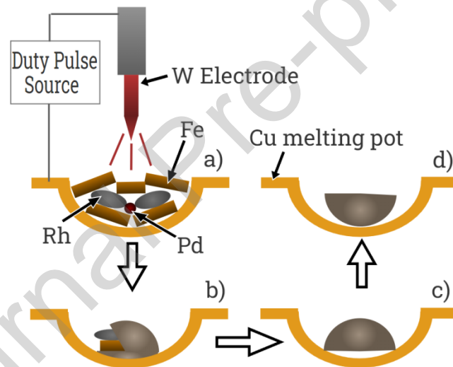
Figure 1. a) The scheme of the Fe and Rh ingots arrangement before melting; b-d) illustrate the process of remelting, followed by sample overturning.
