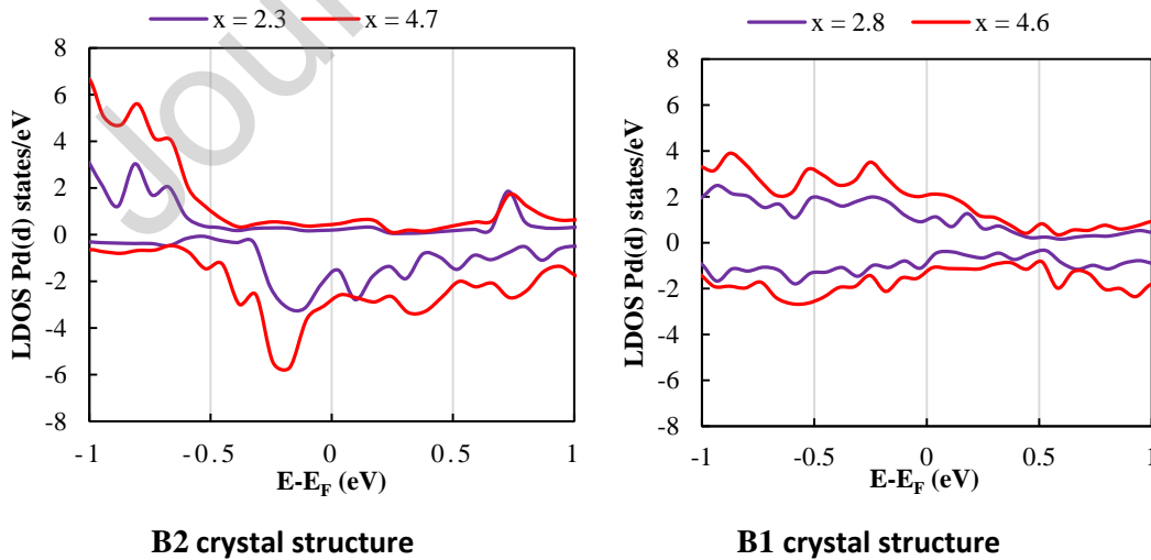
Figure 5 (Color online) Local Pd-4d states in the B2-FM state (left) and B1 -FM states (right) at different contents of Pd. The spin-down (minority) LDOS were plotted as negative values. (For interpretation of the references to color in this figure, the reader is referred to the web version of this article)
