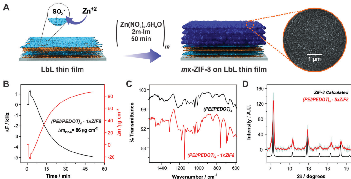
Fig. 2 (A) Schematic showing the deposition of the MOF films onto the LbL-modified substrates, together with a SEM picture of a 3x-ZIF-8-(PEI/PEDOT) 4 substrate. (B) Frequency and mass changes measured by QCM for one ZIF-8 deposition cycle onto a 4 bilayer-modified gold substrate. (C) ATR-FTIR spectra of a (PEI/PEDOT) 4 -modified gold substrate before and after one ZIF-8 deposition cycle. (D) XRD pattern (raw: light green; smoothed: red) of a 5x-ZIF-8-(PEI/PEDOT) 4 -modified substrate.
