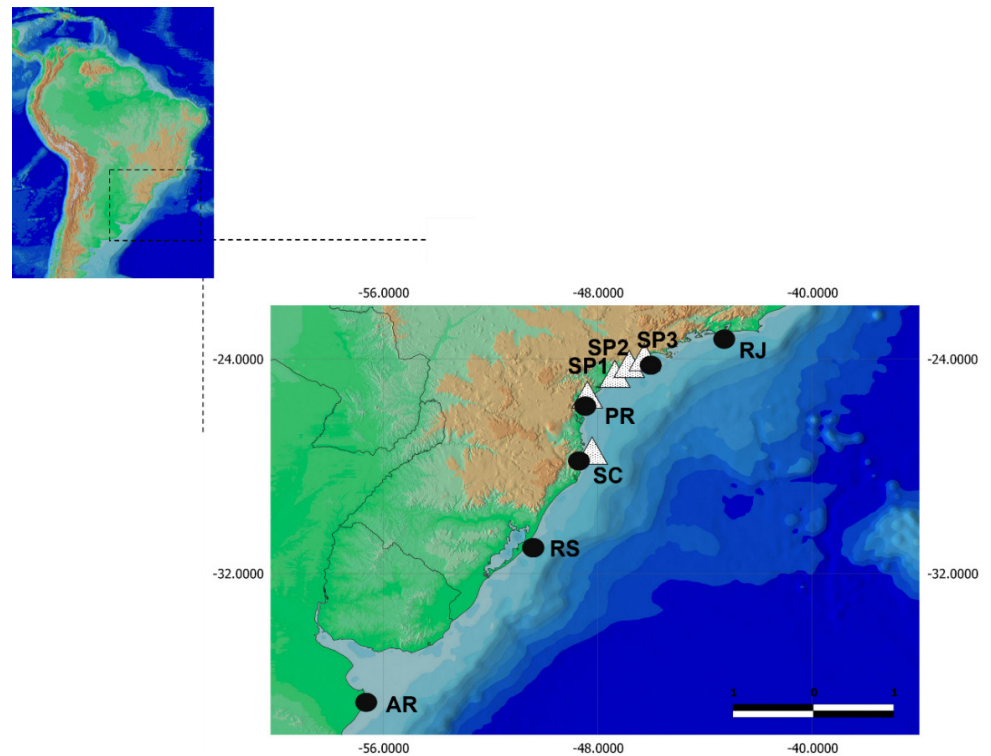
FIGURE 1 | Map showing landing locations of P. horkelii (black circle) and P. percellens (white triangle) in this study. North of Argentina (AR), Rio Grande do Sul (RS), Santa Catarina (SC), Paraná (PR), Cananéia – SP (SP1), Mongaguá – SP (SP2), Santos – SP (SP3), Rio de Janeiro (RJ).
