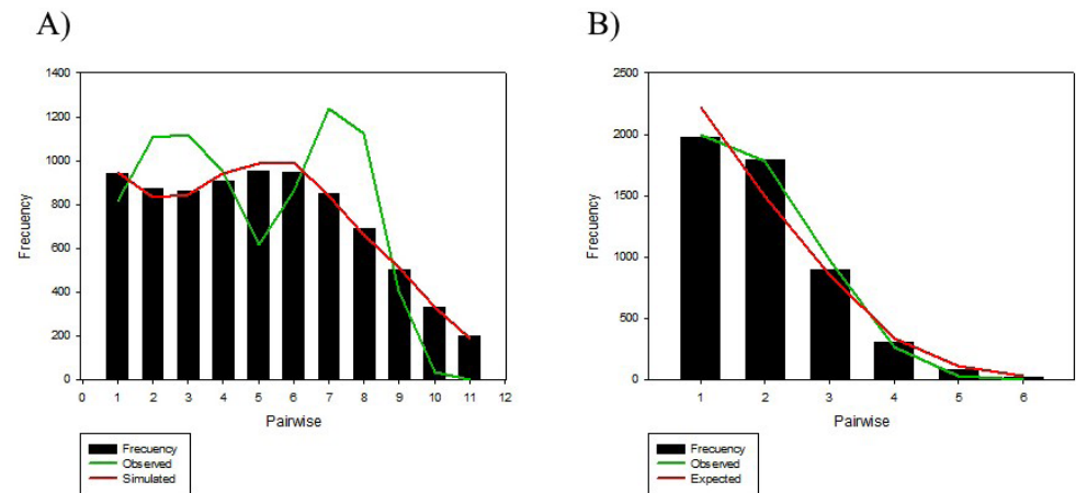
FIGURE 1 | Distribution of mismatches for the Pseudobatos horkelii (A) and P. percellens (B).
