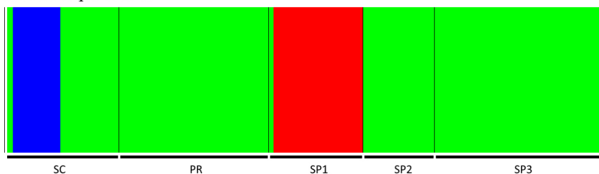
FIGURE 2 | Graph of the Bayesian analysis of population structure of mtCR for A. Pseudobatos horkelii and B. Pseudobatos percellens . Sampled from the northern Argentina (AR), Torrinhã/RS (RS), Florianópolis/SC (SC), Pontal do Paraná/PR (PR), Cananéia/ SP (SP1), Mongaguá/SP (SP2), Santos/SP (SP3), Rio de Janeiro/RJ(RJ).
