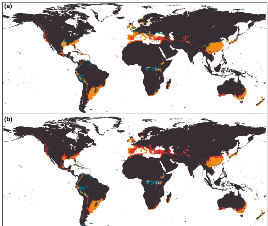
FIGURE 4 Change in suitability pattern of Ligustrum lucidum for the 2050 (a) and 2080 periods (b) assuming a RCP 8.5. Colours depict different types of distribution changes regarding current conditions, orange: stable areas, red: potential distribution lost, blue: potential distribution gains. Grid-cells considered as model extrapolation were eliminated based on MOP analysis in future suitability projection
