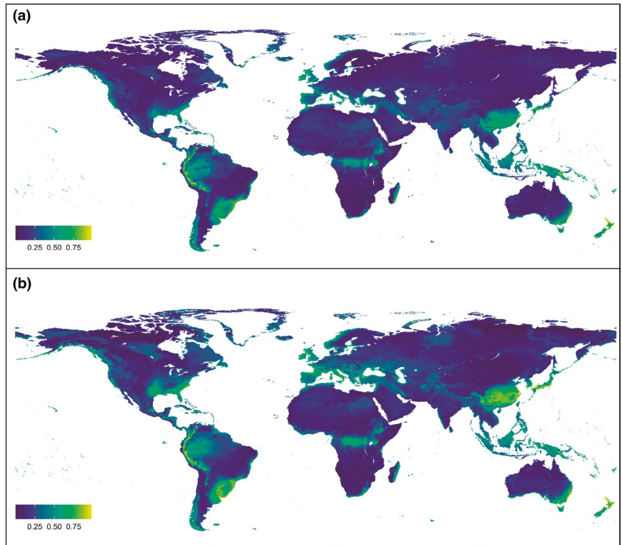
FIGURE 3 Future suitability pattern of Ligustrum lucidum for the periods 2050 (a) and 2080 (b) assuming a RCP 8.5. These models were based on the ensemble of four algorithms and five AOGCMs. Habitat suitability in panel range from 0 to 1
