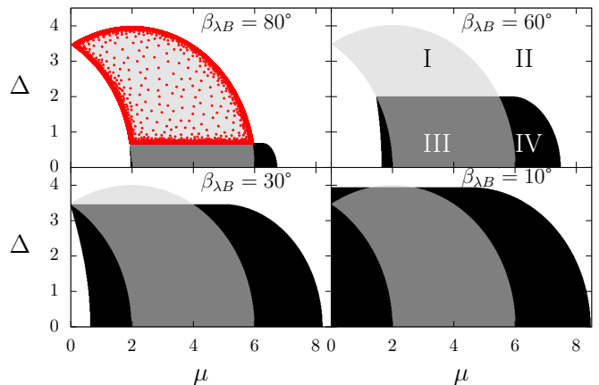
FIG. 2. (Color online) Phase diagram in the \mu, \Delta plane for t = 1 , \lambda = 2 , B = 4 and several values of the angle \beta_{\lambda B} between \vec{\lambda} and \vec{B} . Regions I and II as in Fig. 1. Region III (IV) in dark gray (black) corresponds to the gapless phase with Berry phase \pi (0). The red points at the top left corresponds to numerical calculations which detected localized states at the ends.
