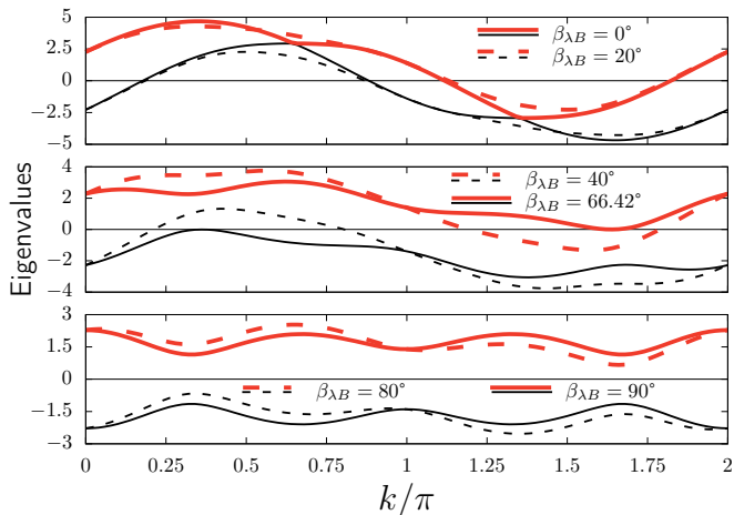
FIG. 3. (Color online) Second (black thin lines) and third (red thick lines) eigenvalues of H_k as a function of wave vector for t = 1 , \lambda = \Delta = 2 , B = \mu = 5 and several values of the angle \beta_{\lambda B} between \vec{\lambda} and \vec{B} .
