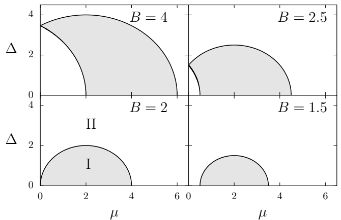
FIG. 1. Phase diagram in the \mu, \Delta plane for perpendicular \vec{\lambda} and \vec{B} , t = 1 , \lambda = |\vec{\lambda}| = 2 , and several values of B . Gray region I denotes the topological sector and white region II the non topological one.
