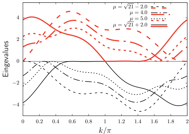
FIG. 4. (Color online) Same as Fig. 3 for t = 1 , \lambda = \Delta = 2 , B = 5 , \beta_{\lambda B} = 66.42^\circ and several values of \mu .
