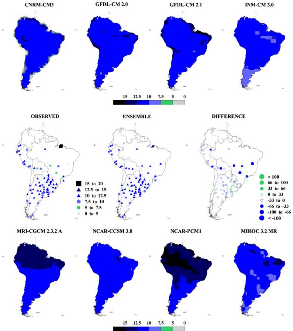
Fig. 1 Mean values of warm nights ( T_{n90} ) for the period 1961–2000, units are percentage over the observation. GCM outputs ( top and bottom lines ), observed, ensemble means and their difference, observed minus ensemble ( center )
