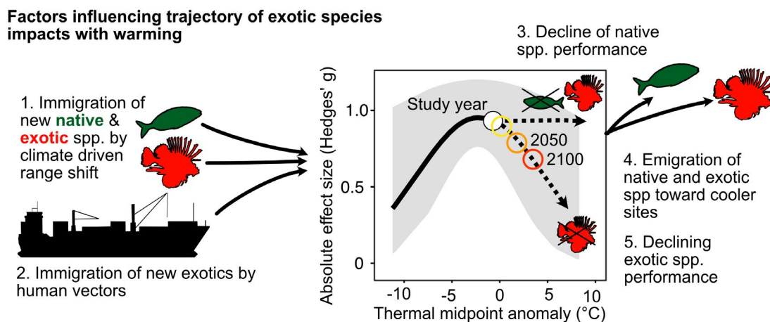
FIGURE 3 Heuristic model of factors influencing the trajectory of impacts of exotic species through time, in response to warming. The graph illustrates the best-fitting model of impacts on the abundance of native taxa in response to thermal midpoint anomalies (Figure 2). The white-filled circle represents the median thermal midpoint anomalies experienced by exotic species at the time studies were conducted. The yellow, orange and red open circles represent median midpoint anomalies in 2020, 2050 and 2100 under RCP8.5 warming projections and the corresponding median projected effect size, based on changes in temperature. However, temporal dynamics of the impacts of exotic species might be influenced by several factors in addition to temperature that might cause impacts to increase, remain stable or decrease through time. These include but are not limited to: immigration of new thermally tolerant native and new exotic species into the recipient site (1, 2); relative differences in thermal sensitivity between interacting native and exotic species in response to warming (3, 5); and poleward movement of established native and exotic species from recipient sites toward cooler sites (4) [Colour figure can be viewed at wileyonlinelibrary.com ]
