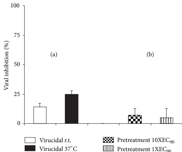
FIGURE 3: Virucidal activity (a) and the effect of pretreatment of Vero cells with euparin (b). The virucidal activity of 10 \mu\text{g}/\text{mL} (10X EC 90 ) at 37°C and r.t. and the pretreatment with 1.0 and 10 \mu\text{g}/\text{mL} were evaluated against PV-1. Data represent % of virus inhibition compared to untreated controls as mean \pm SD ( n = 3 ). Experiments were done in quadruplicate.
