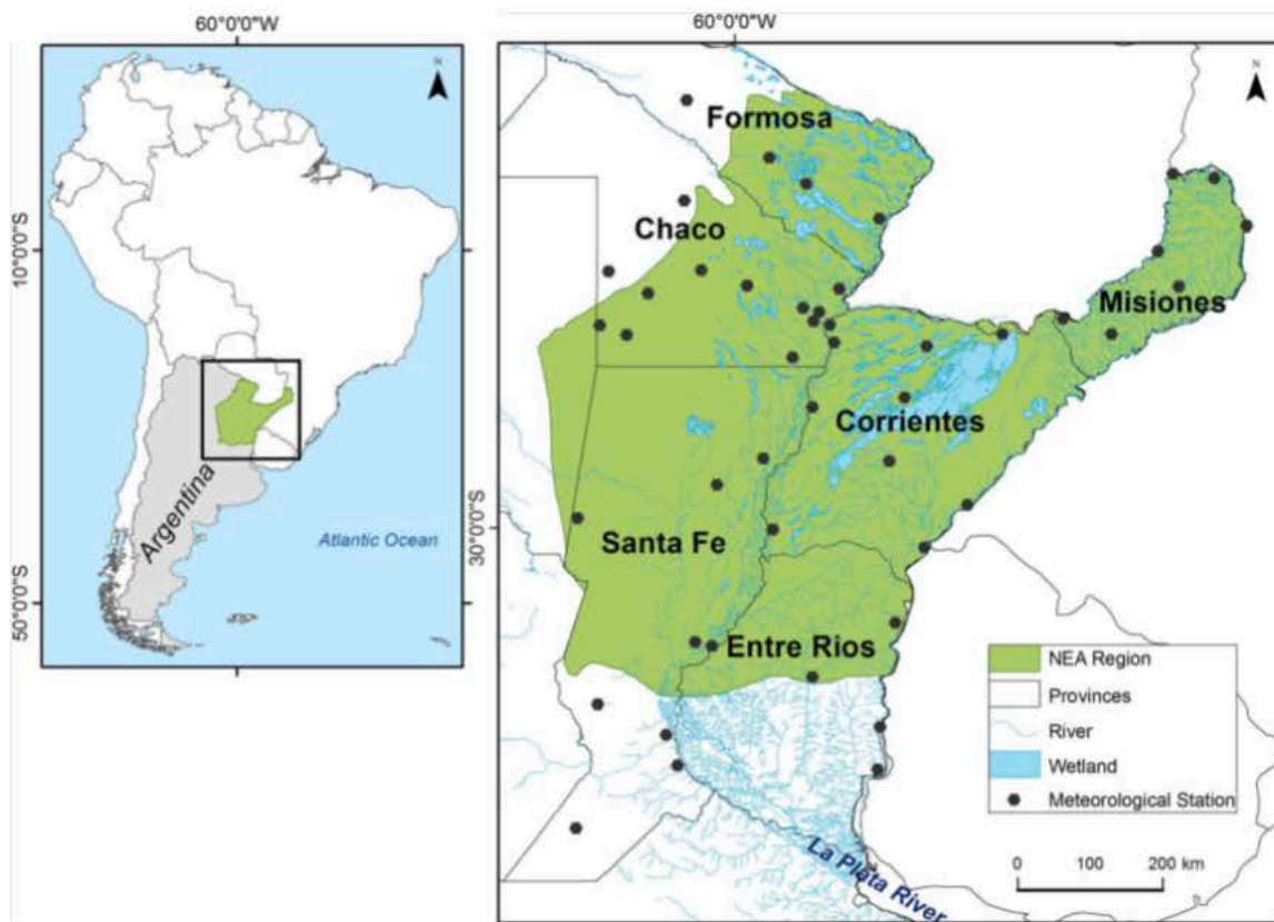
Fig. 1 The NEA region (Argentina) in the southeast of South America; its main rivers, wetlands, and meteorological stations were chosen considering record length and completeness
