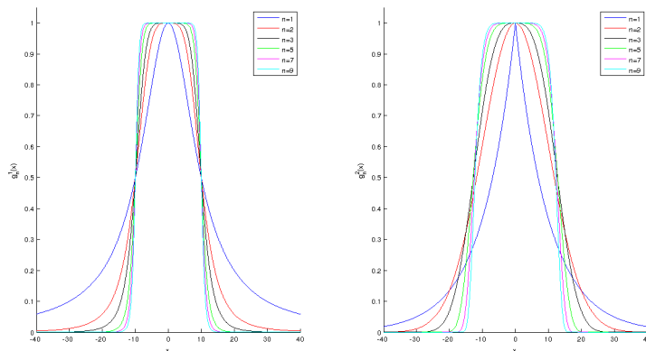
Fig. 1. Plot of g_n^1(x) = \frac{1}{1+x^2n/102n} and g_n^2(x) = e^{\left(\frac{-|x|^n}{n10^n}\right)} for different values of n
