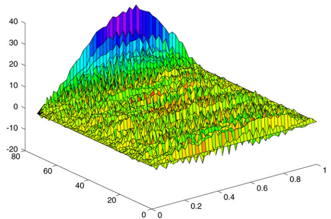
Fig. 3. The graph of a sample solution with initial datum u_0 \equiv 0 .
