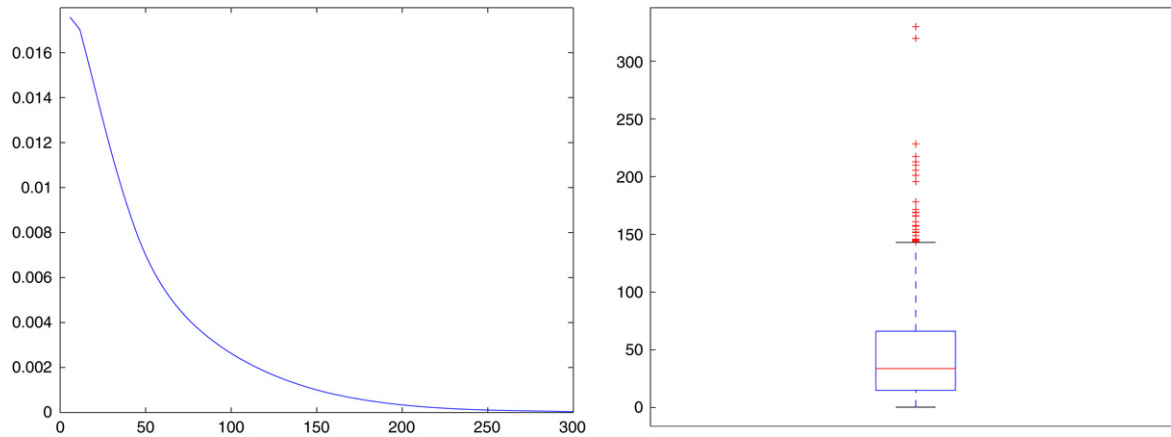
Fig. 4. The kernel density estimator of the explosion time for \sigma = 6.36 and the corresponding box-plot.
