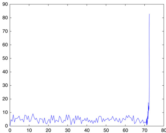
Fig. 2. The evolution of the maximum of a sample solution with initial data u_0 \equiv 0 .
