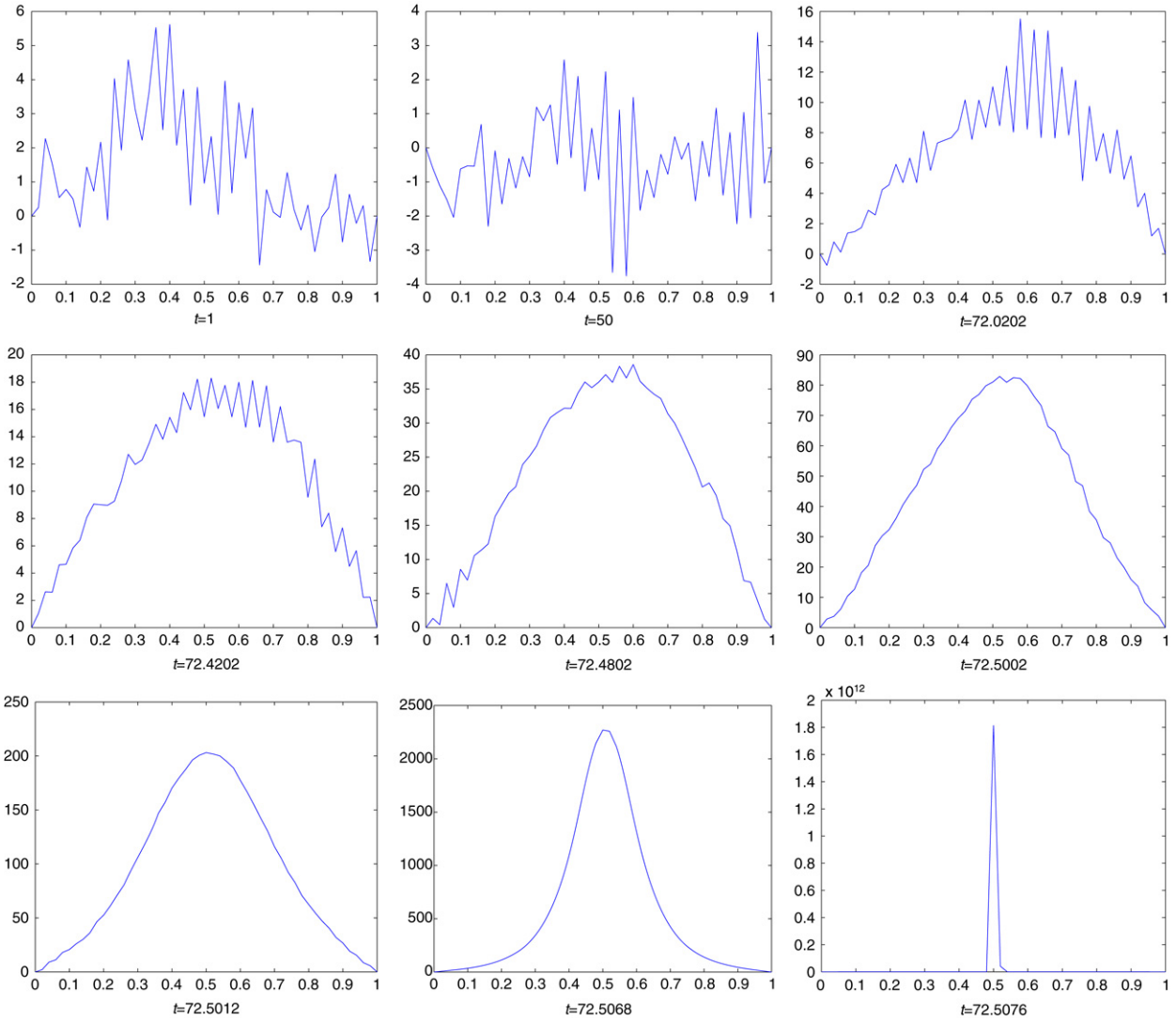
Fig. 1. Profiles of a sample solution at different times.
