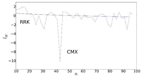
Figure 4. Rate of convergence of the RRK (solid line) and CMX (dashed line) for \omega = 1 , \omega_0 = 1 , g = 5
