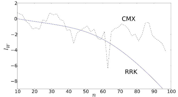
Figure 3. Rate of convergence of the RRK (solid line) and CMX (dashed line) for \omega = 1 , \omega_0 = 1 , g = 2
