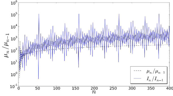
Figure 1. Ratio of moments \mu_n/\mu_{n-1} (dashed line) and of connected moments I_n/I_{n-1} (solid line) for the Rabi Hamiltonian with \omega_0 = \omega = 1 and g = 5 .
