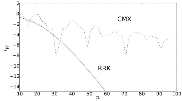
Figure 2. Rate of convergence of the RRK (solid line) and CMX (dashed line) for \omega = 1 , \omega_0 = 1 , g = 1
