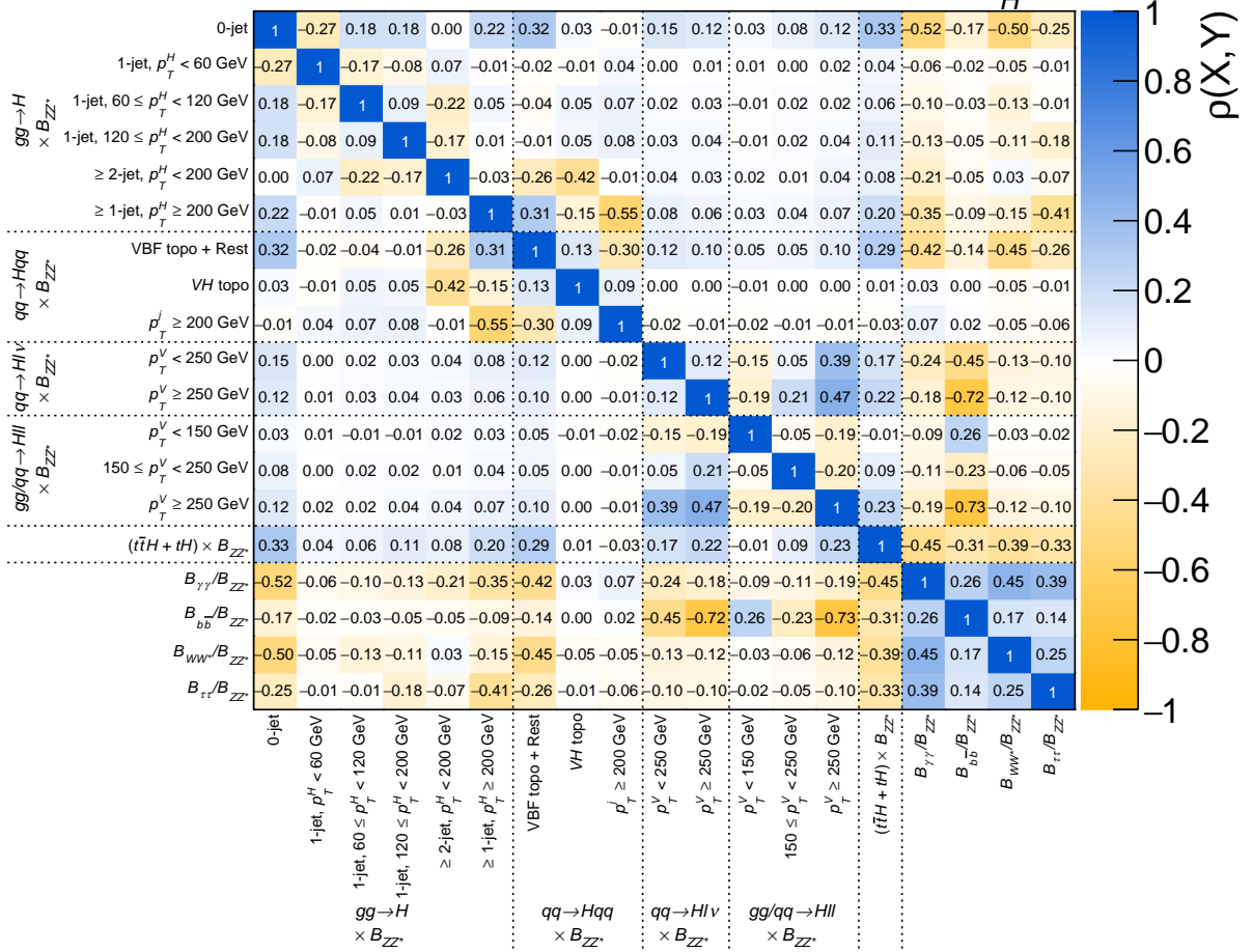
Figure 11: Correlation matrix for the measured values of the simplified template cross sections and ratios of branching fractions. The fit parameters are the products ( \sigma_i \times B_{ZZ}^* ) and the ratios B_f/B_{ZZ}^* .
