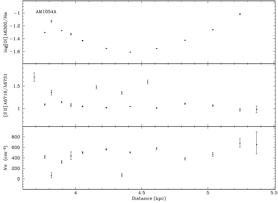
Figure 3. AM 1054-325. \log([O\text{ I}] \lambda 6300/H\alpha) ratio, [S\text{ II}] \lambda 6716/\lambda 6731 ratio and N_e as a function of the galactocentric radius for AM 1054A.
