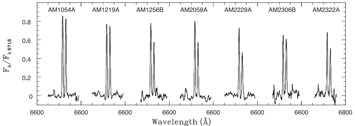
Figure 2. A sample of spectra in the range of 6600–6800 Å from areas of different galaxies. The flux scale was normalized to the peak of [\text{S II}] \lambda 6716 .
