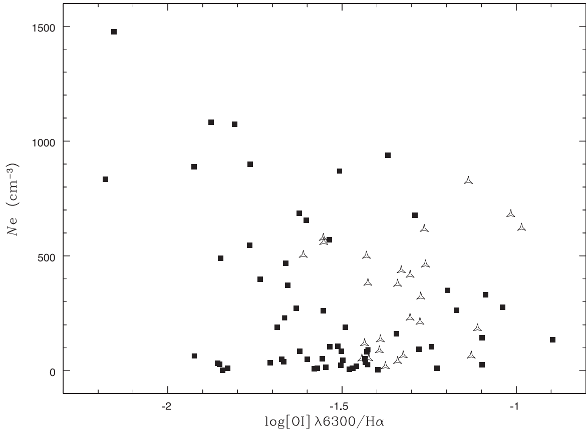
Figure 18. Electron density values N_e derived for our sample versus the observed [O I] \lambda 6300/H\alpha ratio. The squares represent regions ionized by massive stars while the triangles represent those with gas shock excitation, according to the diagnostic diagram presented in Fig. 17.
