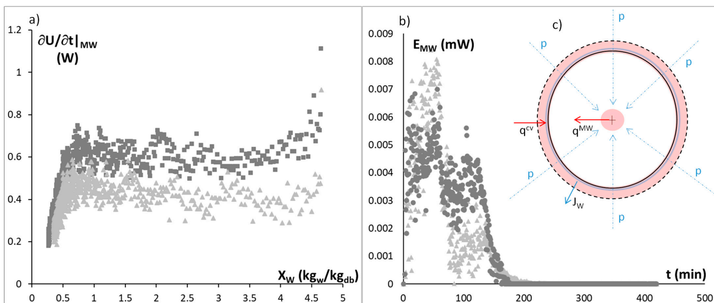
Figure 8. (a) Internal energy accumulation throughout the drying time for HAD + 4 W/g ( \blacktriangle ) and HAD + 6 W/g ( \blacksquare ) treatments, (b) microwave heating of the boundary layer throughout the drying time for HAD + 4 W/g ( \blacktriangle ) and HAD + 6 W/g ( \blacksquare ) treatments. (c) Scheme of the effect of microwaves in sample heating, where p represents the photon fluxes, q^{MW} represents the heat conduction produced by the microwave heating source in the sample center, J_w is the water flux and q^{cv} is the heat convection.
