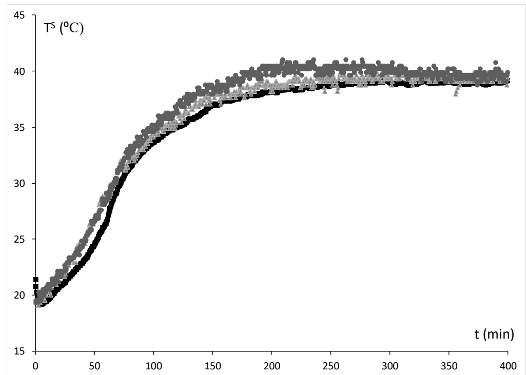
Figure 4. Evolution of surface temperature in the HAD treatment (■), HAD + 4 W/g treatment (▲) and HAD + 6 W/g treatment (●).
