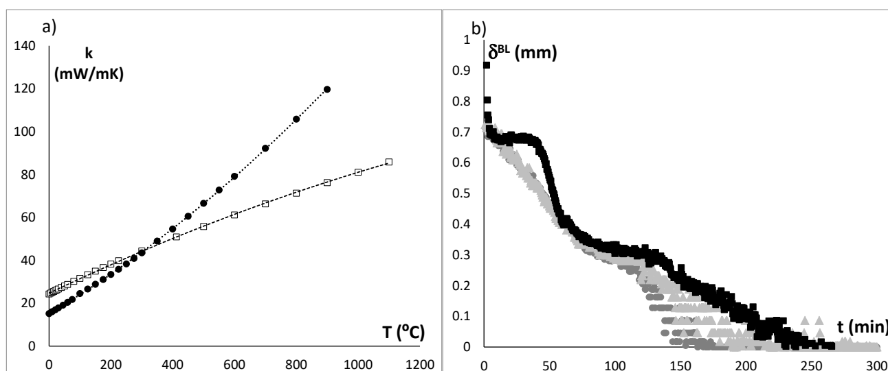
Figure 6. (a) Plot of the thermal conductivity of dry air (●) and vapor (□) with regards to the temperature and (b) plot of the boundary layer depth with regards to the drying time: HAD treatment (■), HAD + 4 W/g treatment (▲) and HAD + 6 W/g treatment (●).
