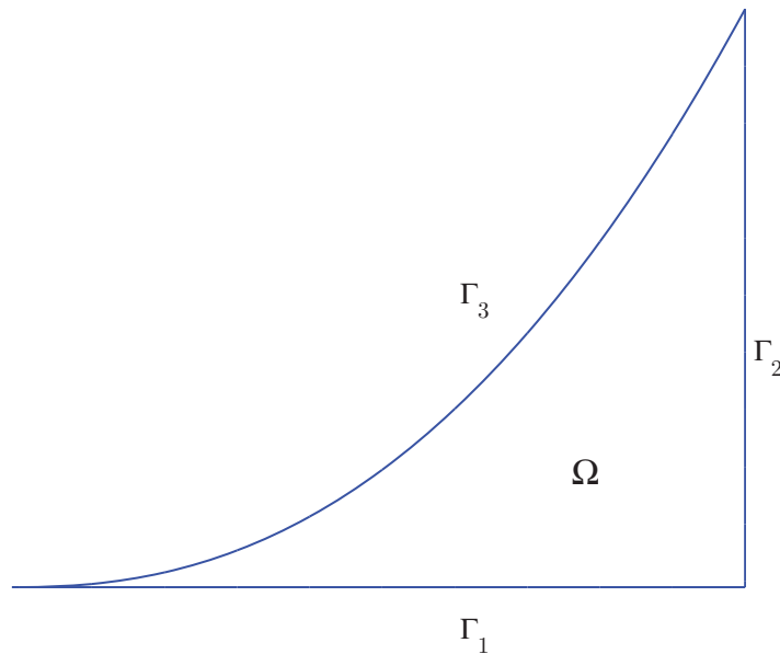
FIGURE 1. Cuspidal domain
