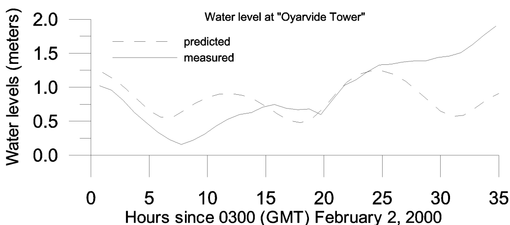
Figure 5. Observed sea levels gathered in "Oyarvide Tower" (solid) and predicted tide (meters).
