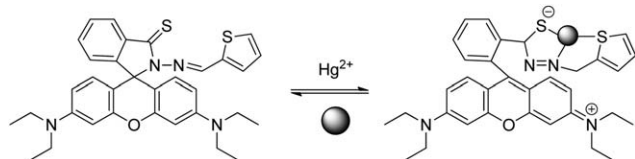
Scheme 15 Proposed binding mode of RB13 with \text{Hg}^{2+} .
